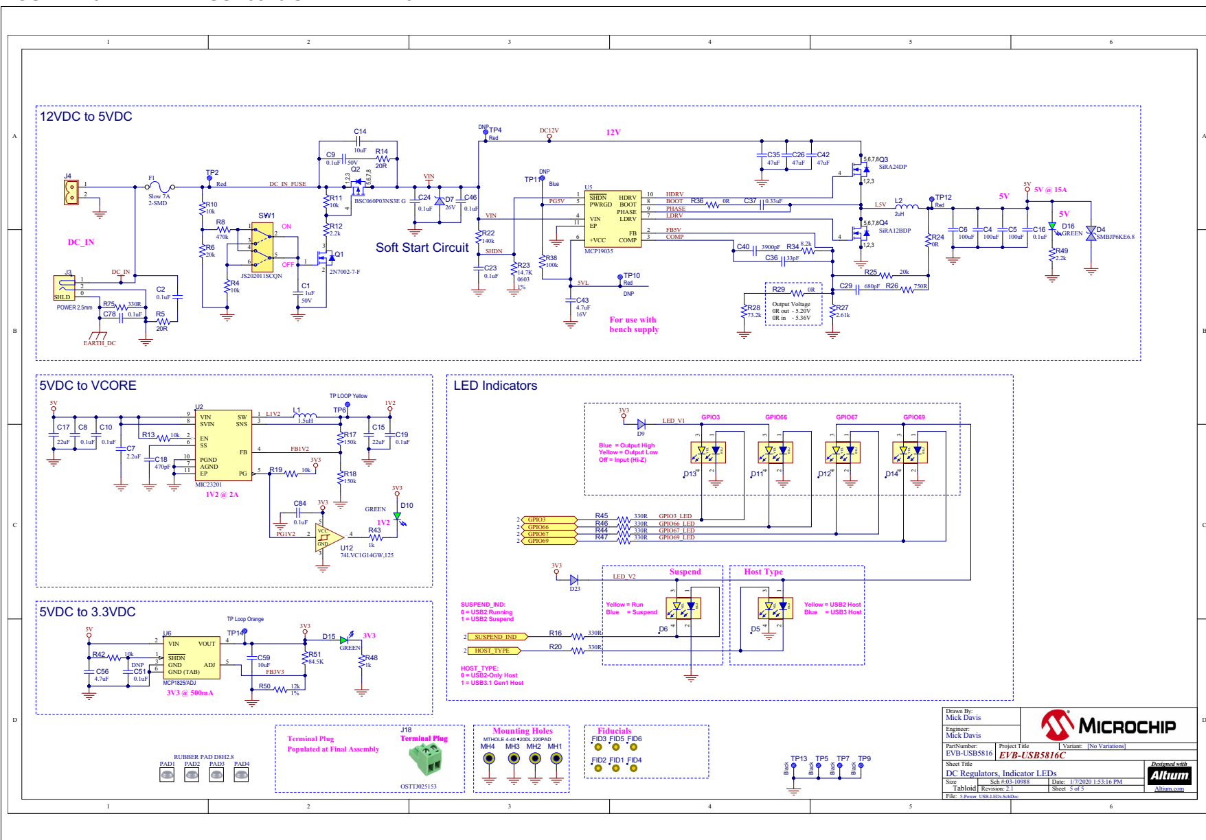
FIGURE A-5: EVB-USB5816 SCHEMATIC 5
