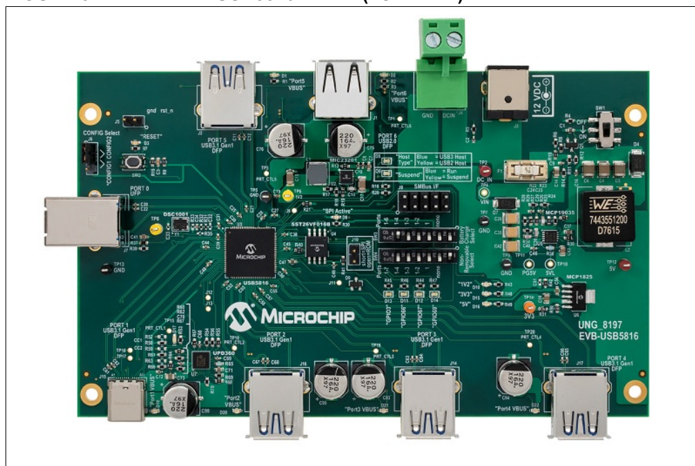
FIGURE 3-1: EVB-USB5816 REV B (TOP VIEW)
