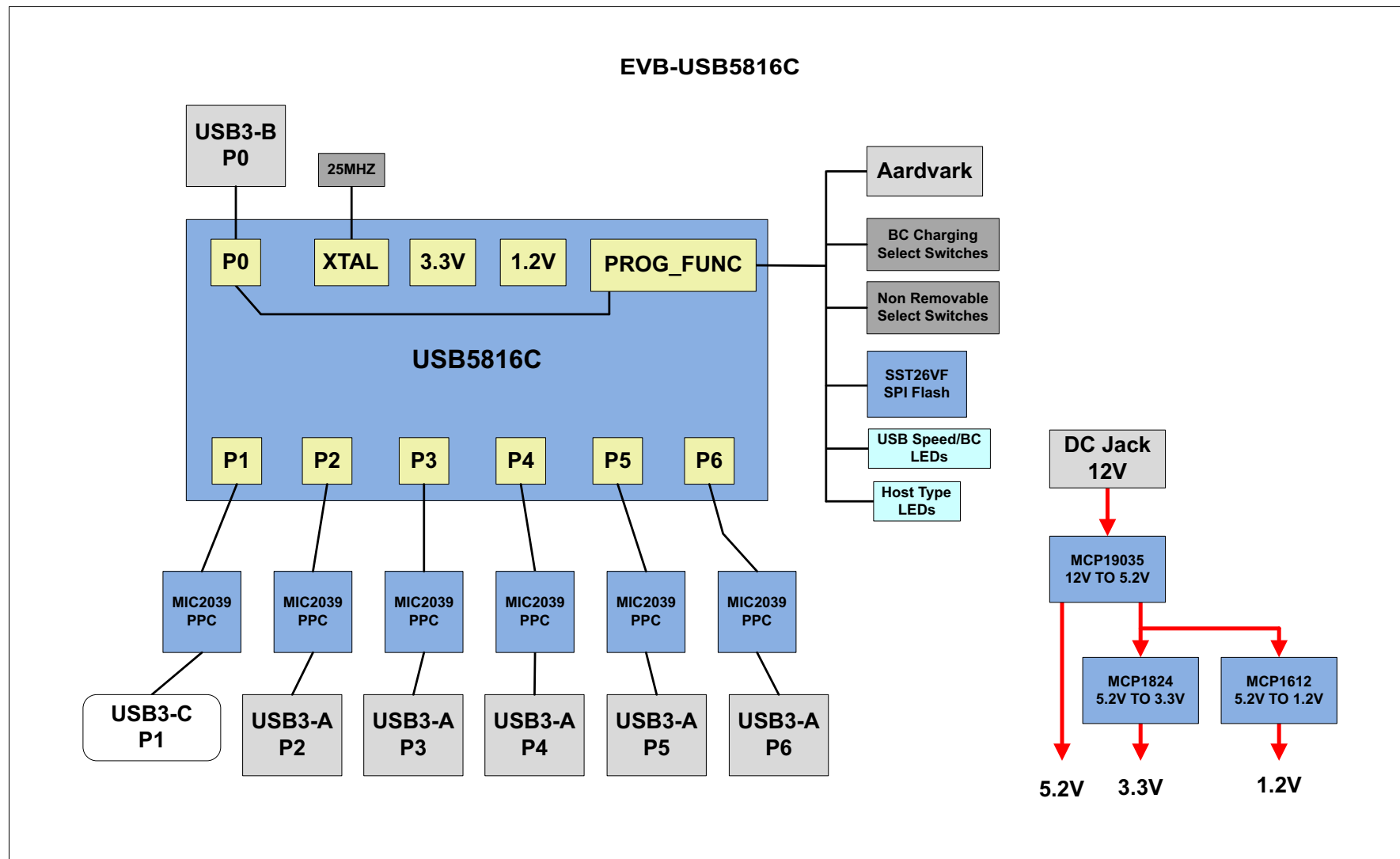
FIGURE 1-1: BLOCK DIAGRAM
