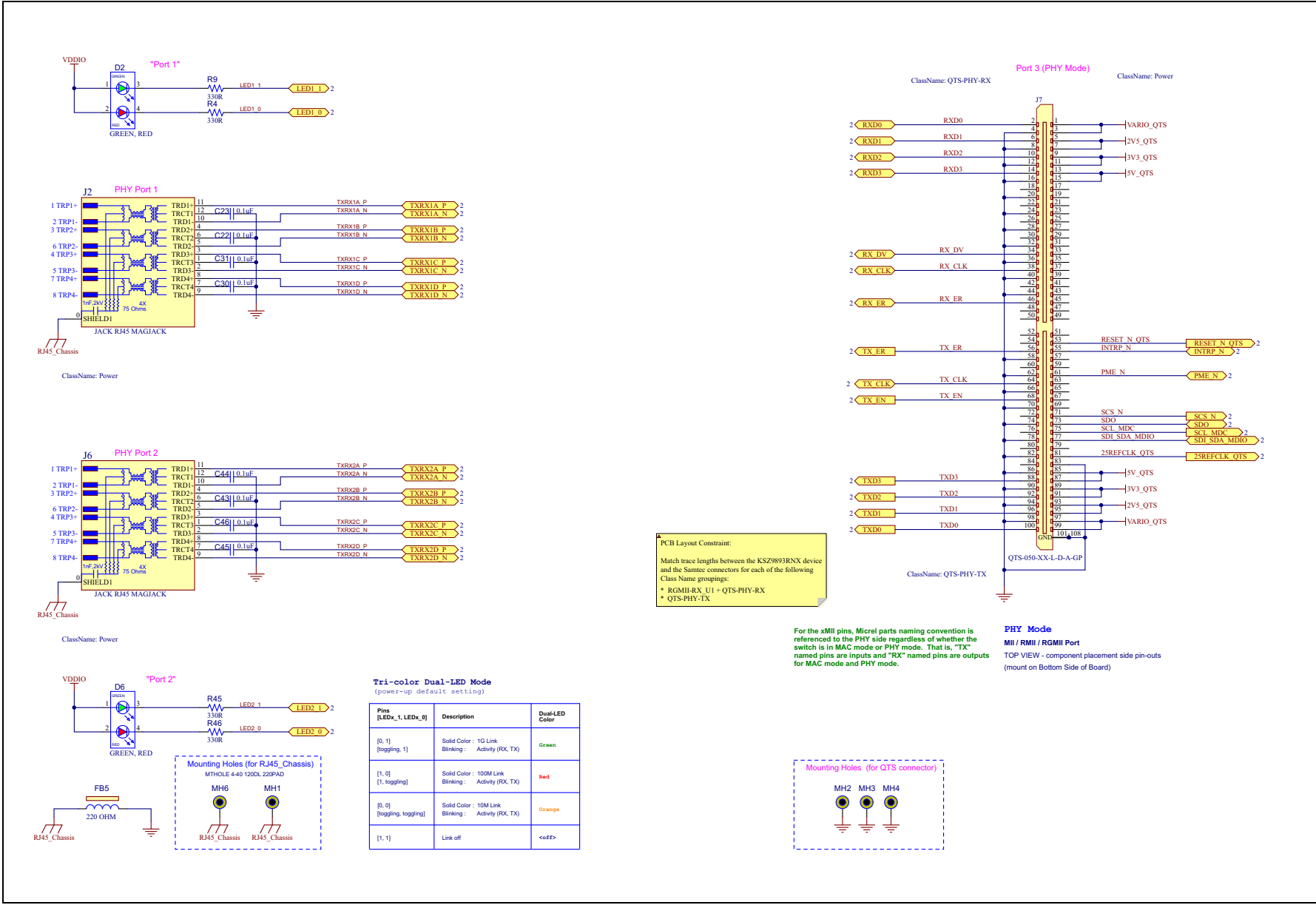
FIGURE B-2: EVB-KSZ9893 SCHEMATICS – PORTS 1 AND 2 PHYS; PORT 3 MAC – MII/RMII/RGMII CONNECTOR
