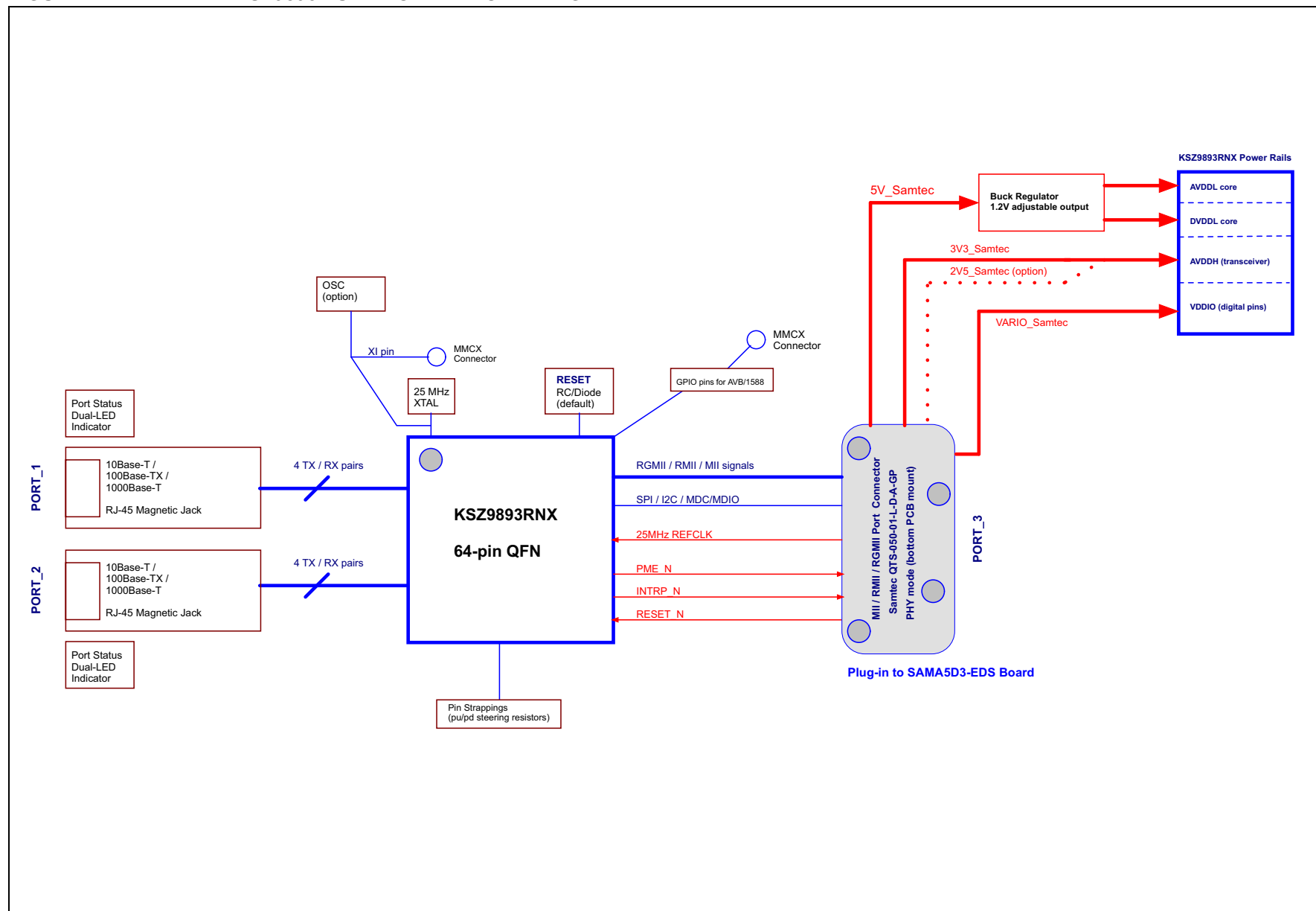
FIGURE 1-1: EVB-KSZ9893 FUNCTIONAL BLOCK DIAGRAM
