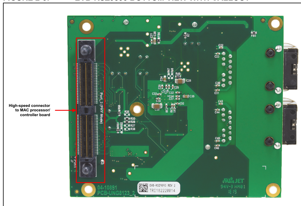
FIGURE 2-3: EVB-KSZ9893 BOTTOM VIEW WITH CALLOUT
