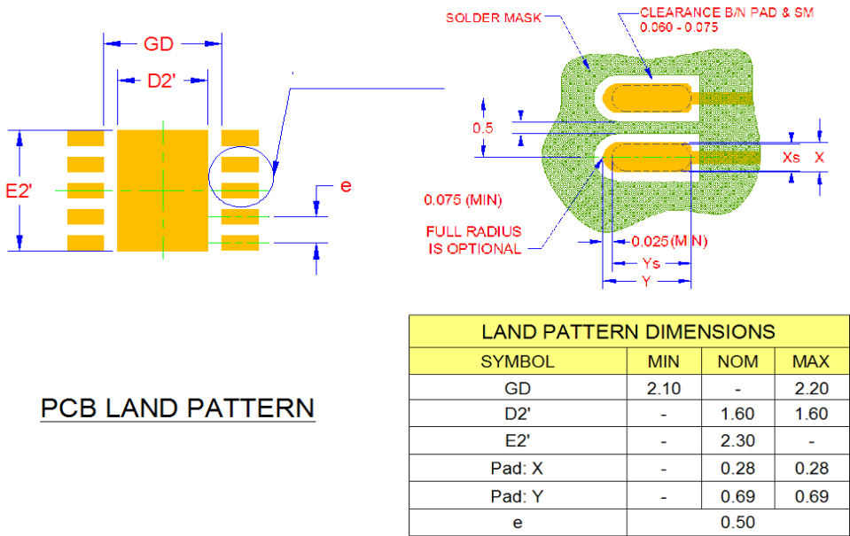
Figure 8.3 10 Pin DFN PCB Footprint
