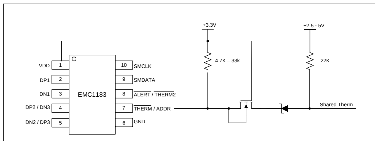
Figure 4.4 Isolating the THERM pin
