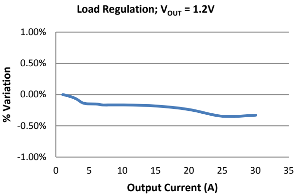
Figure 10. Load Regulation
