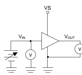
Test Setup 3 Input Threshold Voltage
