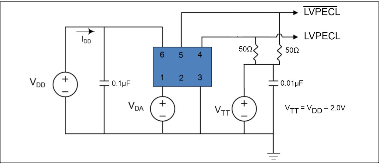
FIGURE 3-5: Test Circuit.
