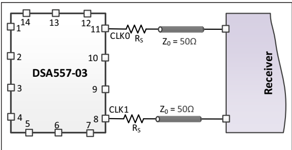
FIGURE 2-3: LVCMOS Outputs.
