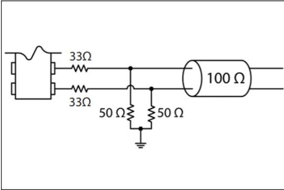
FIGURE 5-3: Typical HCSL Termination Scheme.
