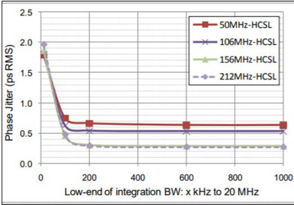
FIGURE 2-4: HCSL Phase Jitter.
