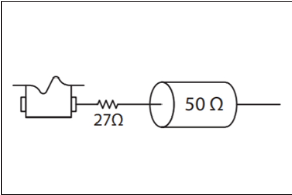
FIGURE 5-4: Typical LVCMOS Termination Scheme.
