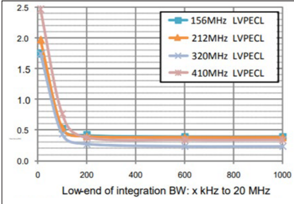
FIGURE 2-3: PECL Phase Jitter.
