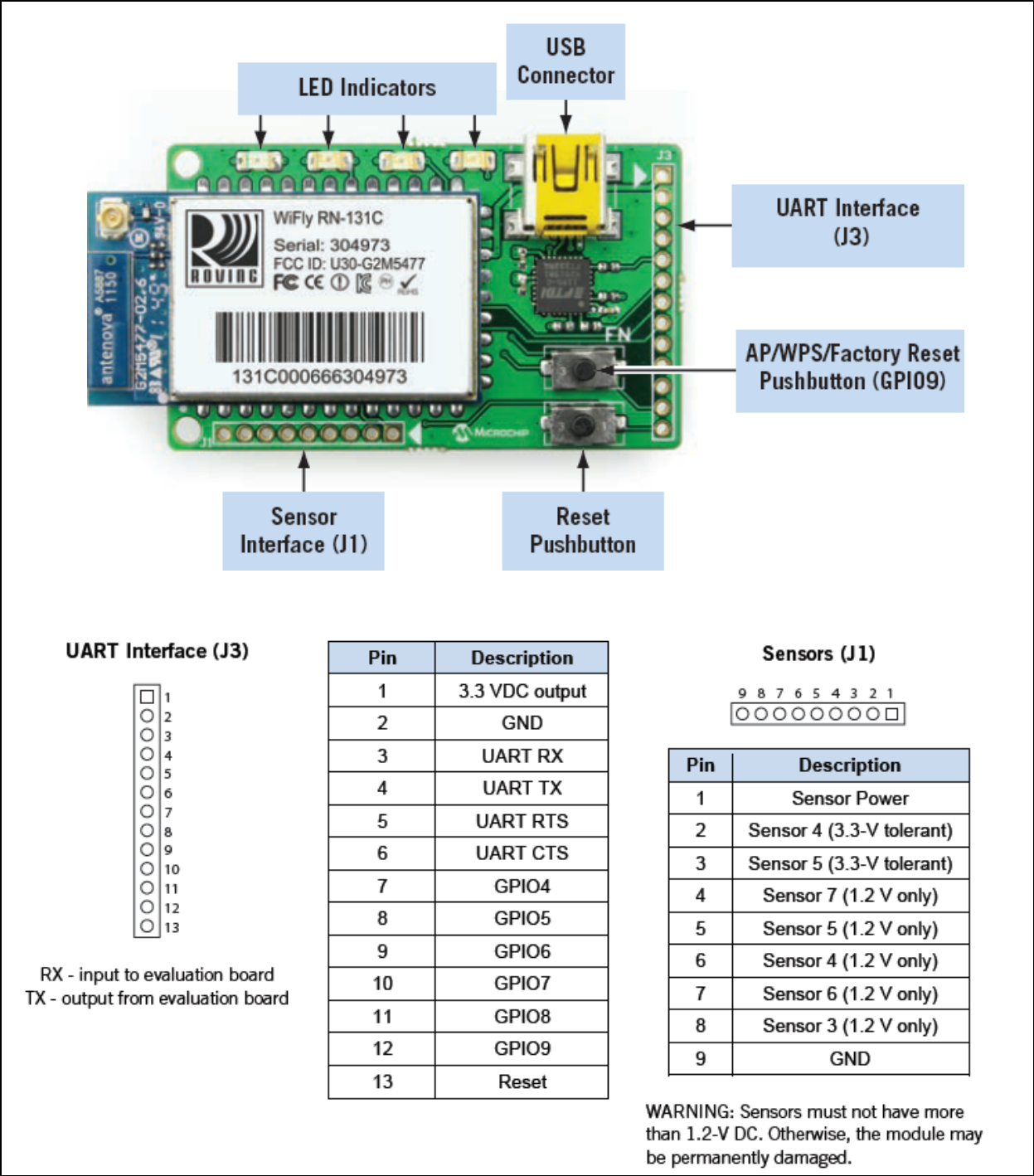
FIGURE 1-2: RN131 EVALUATION BOARD COMPONENTS
