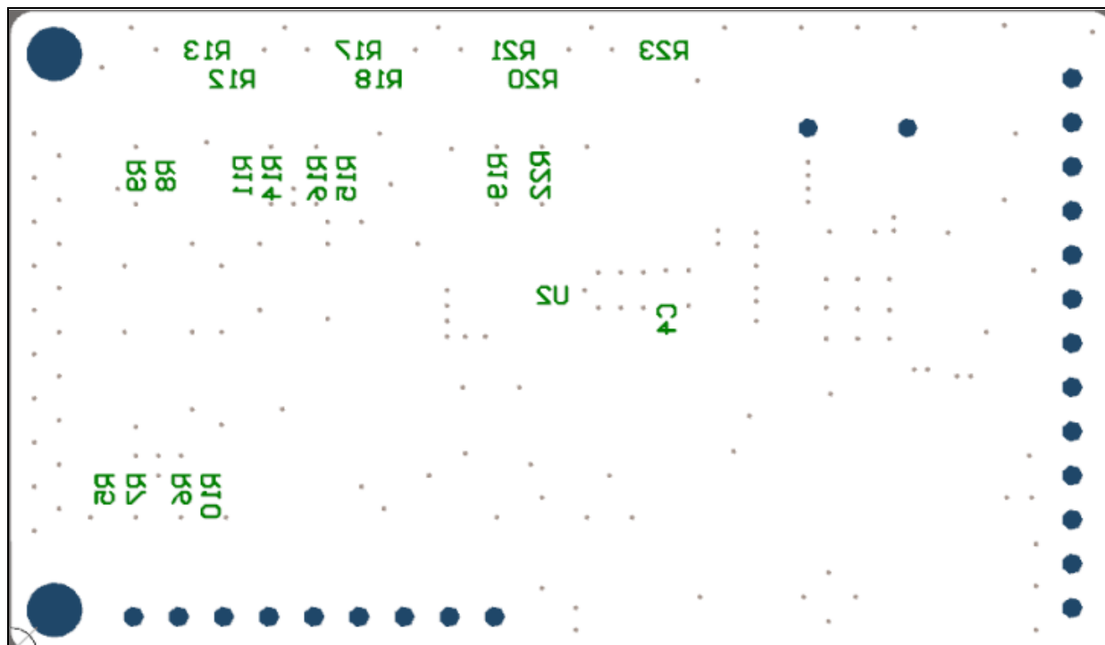
FIGURE A-8: RN131 EVALUATION BOARD BOTTOM ASSEMBLY
