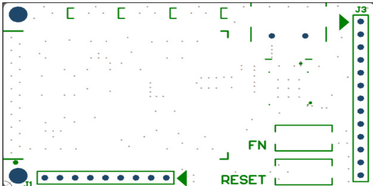
FIGURE A-3: RN131 EVALUATION BOARD TOP SILKSCREEN
