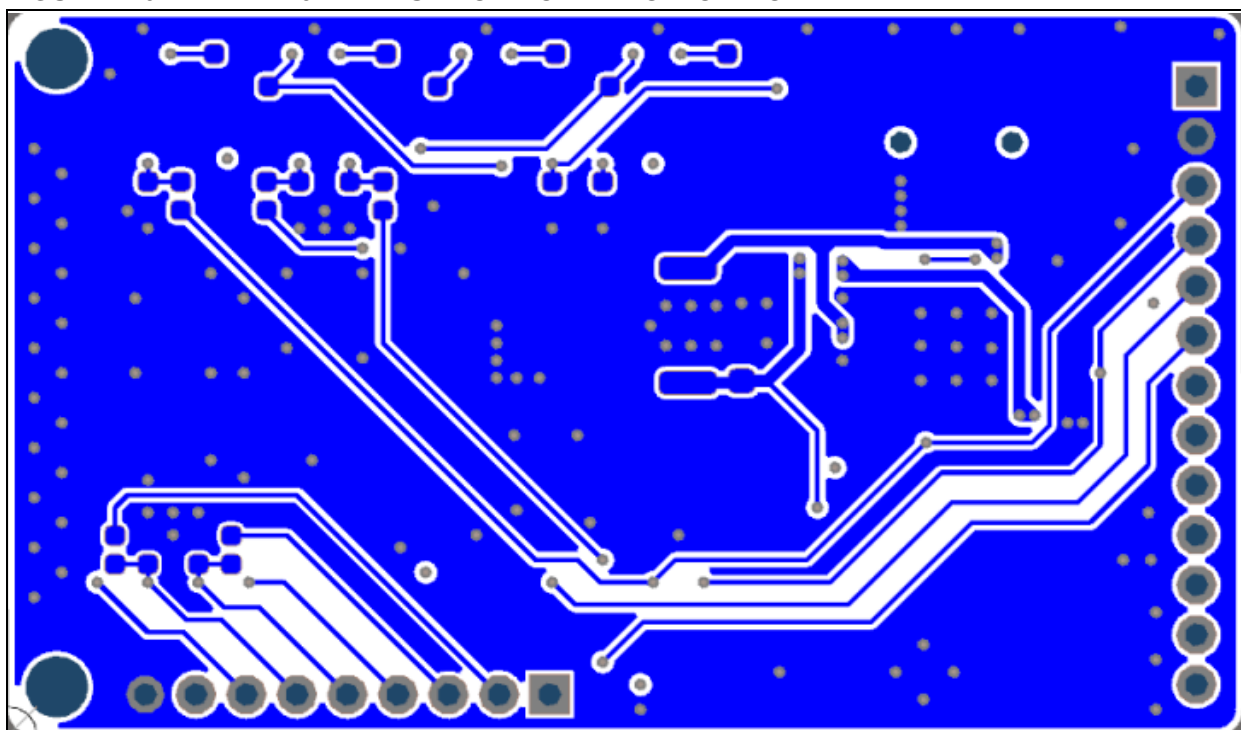
FIGURE A-6: RN131 EVALUATION BOARD BOTTOM COPPER
