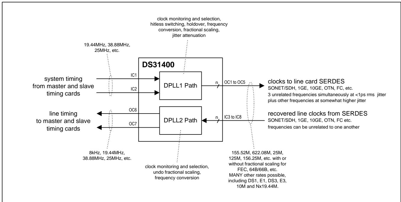
Figure 2-2. Typical Line Card Application Example
