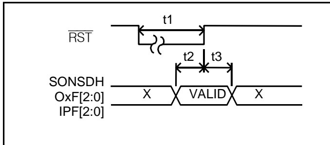
Figure 10-5. Reset Pin Timing Diagram
