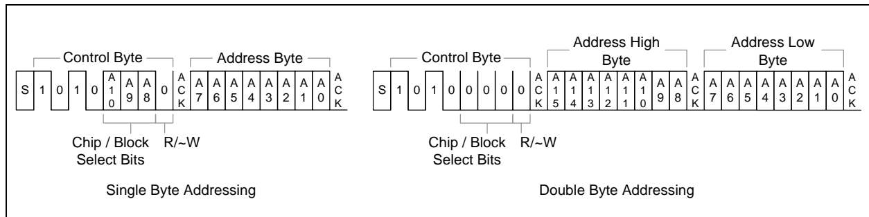
FIGURE 8-3: I 2 C EEPROM ADDRESSING
