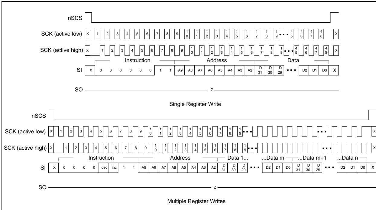
FIGURE 8-16: SPI WRITES
