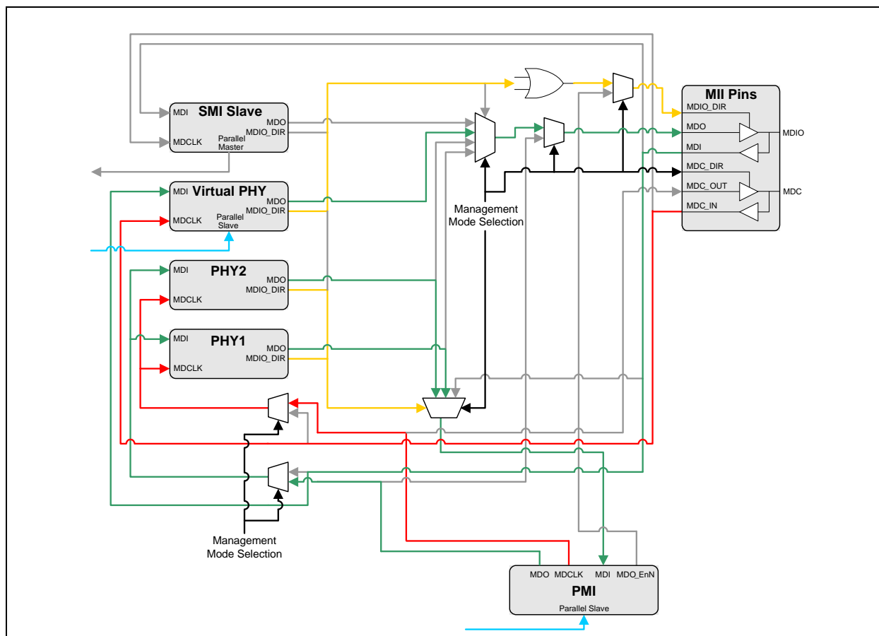
FIGURE 9-6: MII MUX MANAGEMENT PATH CONNECTIONS - PHY MODE I 2 C/SPI MANAGED
