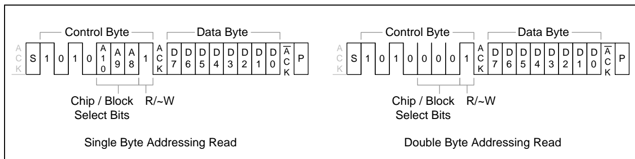
FIGURE 8-4: I 2 C EEPROM BYTE READ
