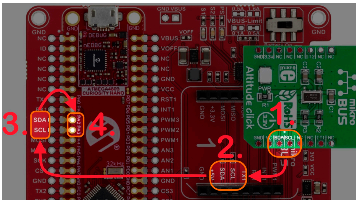
Figure 3-2. Pin Map Example
