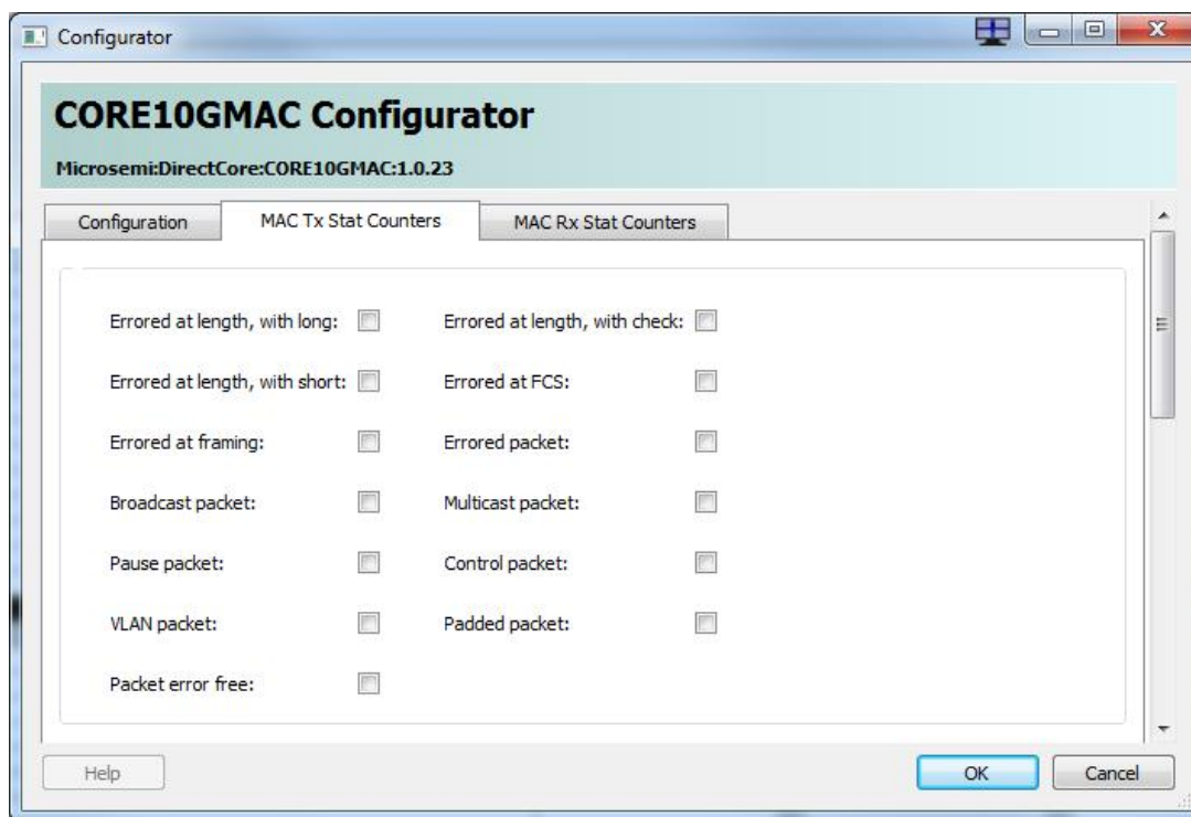
Figure 15 Core10GMAC SmartDesign Configuration GUI (continued)
