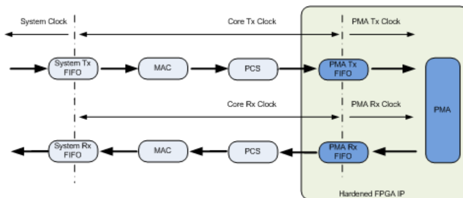
Figure 6 FPGA Clocking Architecture
