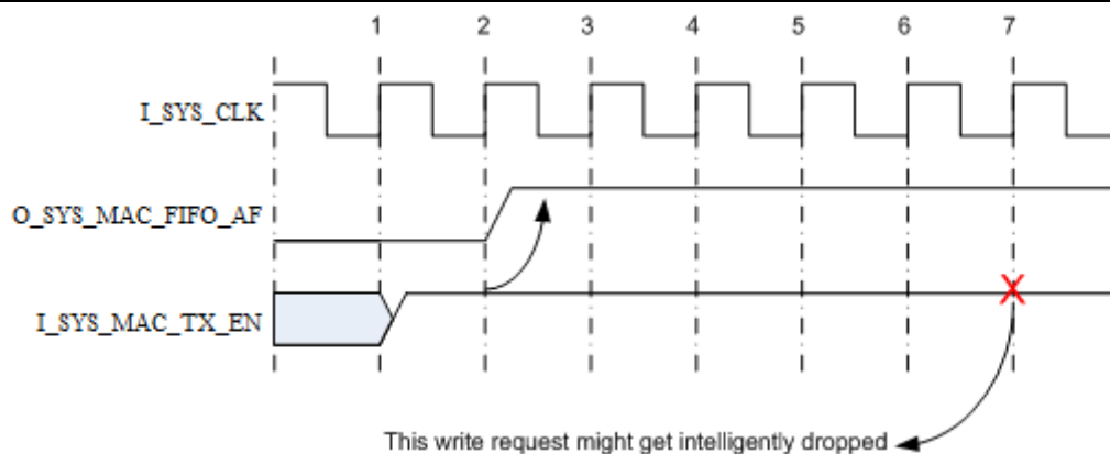
Figure 10 Tx Dataplane Backpressure Timing Diagram
