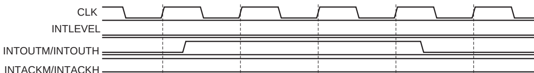
Figure 4-7 • Interrupt Timing (INTLEVEL = 0)
