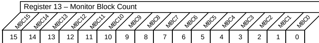
Figure 8-17 • Register 13 – Monitor Block Count
