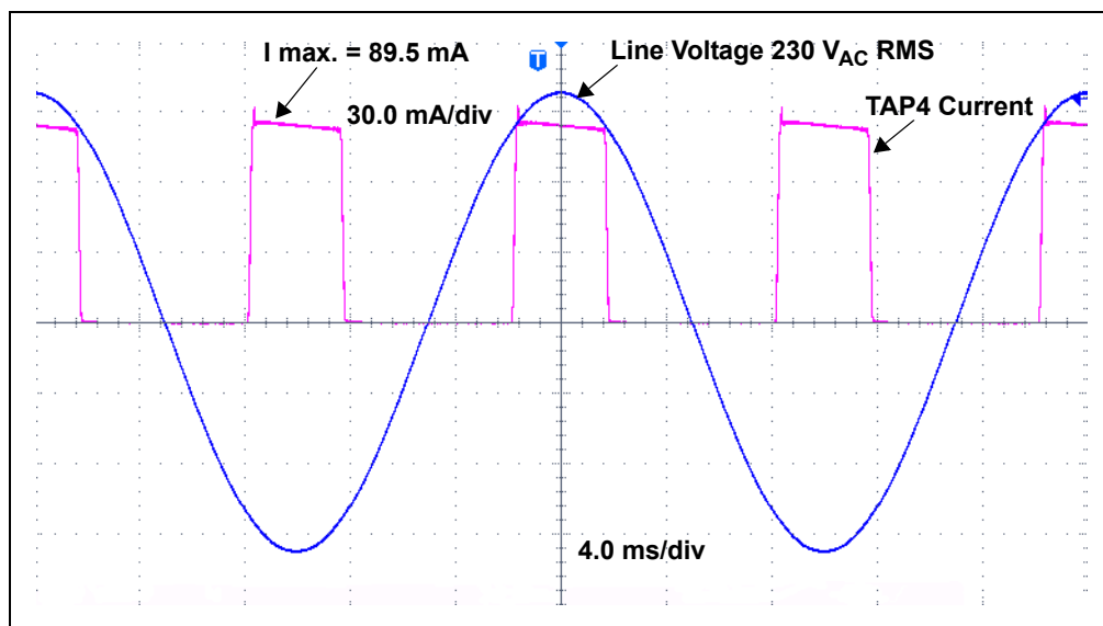
FIGURE C-6: TAP4 Current at 230 V AC Line Input Voltage.
