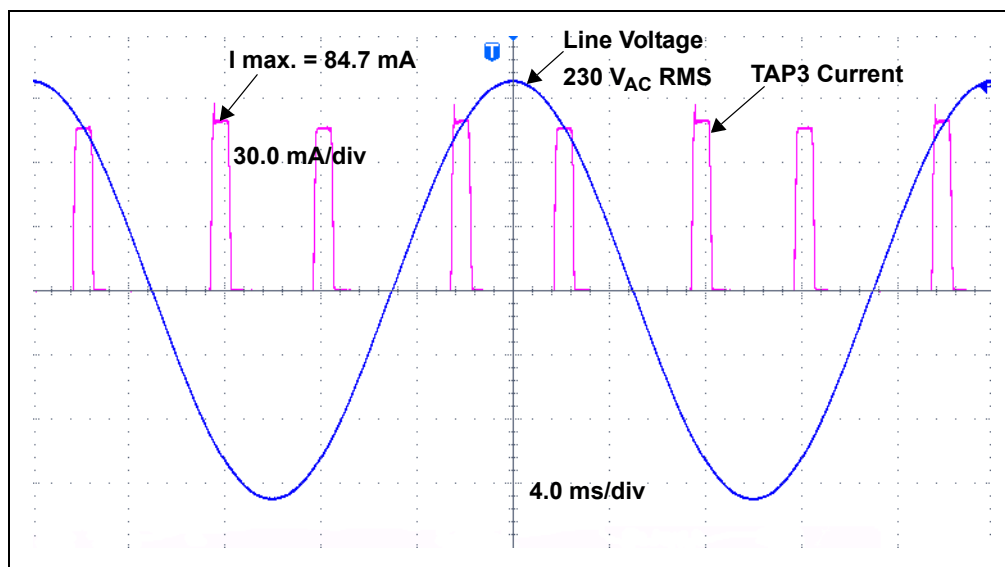
FIGURE C-5: TAP3 Current at 230 V AC Line Input Voltage.
