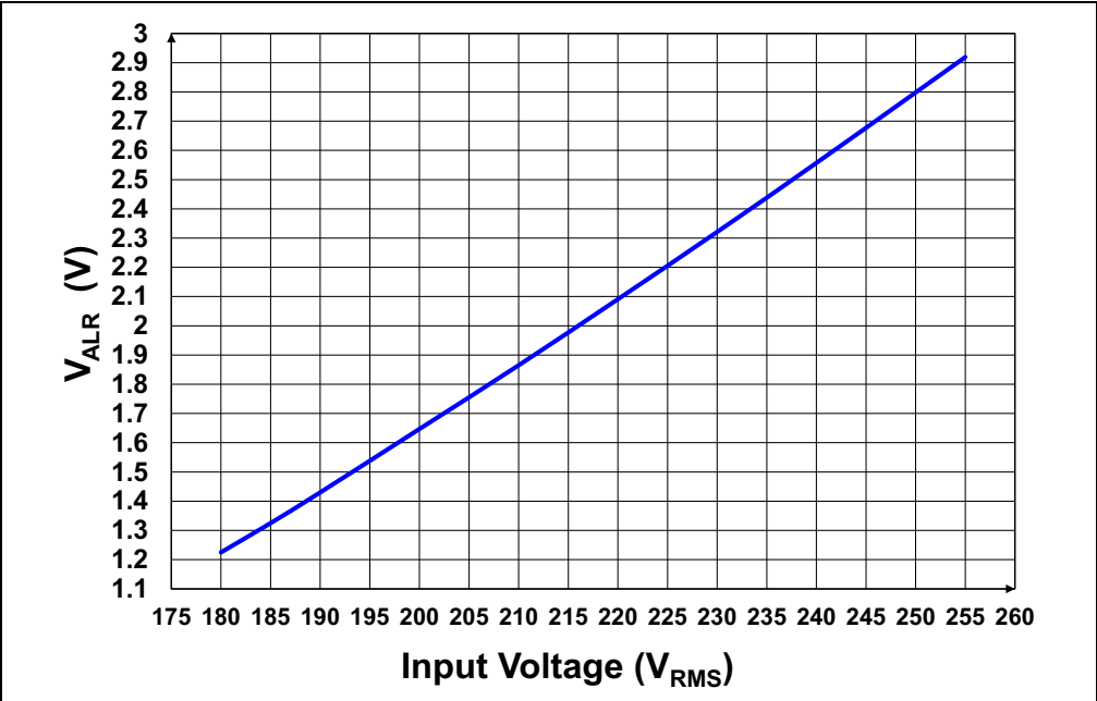
FIGURE C-14: V_{ALR} Pin vs. Input Line Voltage ( V_{RMS} ).
