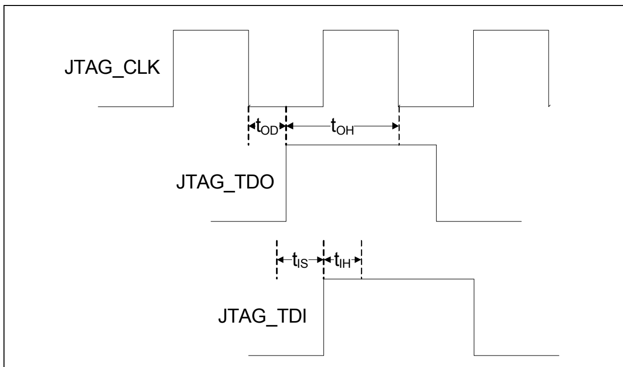
FIGURE 39-23: JTAG SETUP &amp; HOLD PARAMETERS
