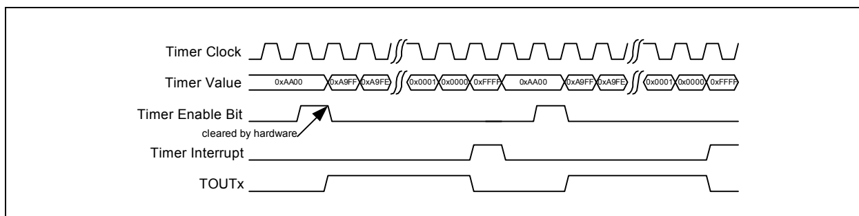
FIGURE 14-10: ONE SHOT TIMER WITH PULSE OUTPUT
