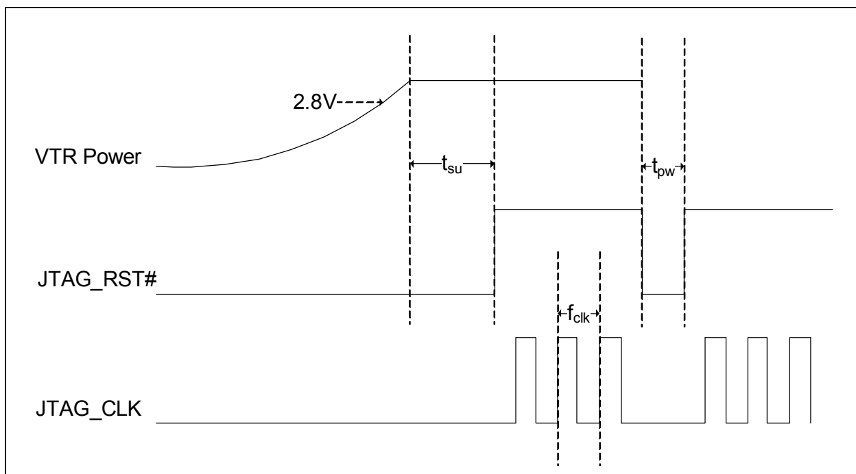
FIGURE 39-22: JTAG POWER-UP &amp; ASYNCHRONOUS RESET TIMING
