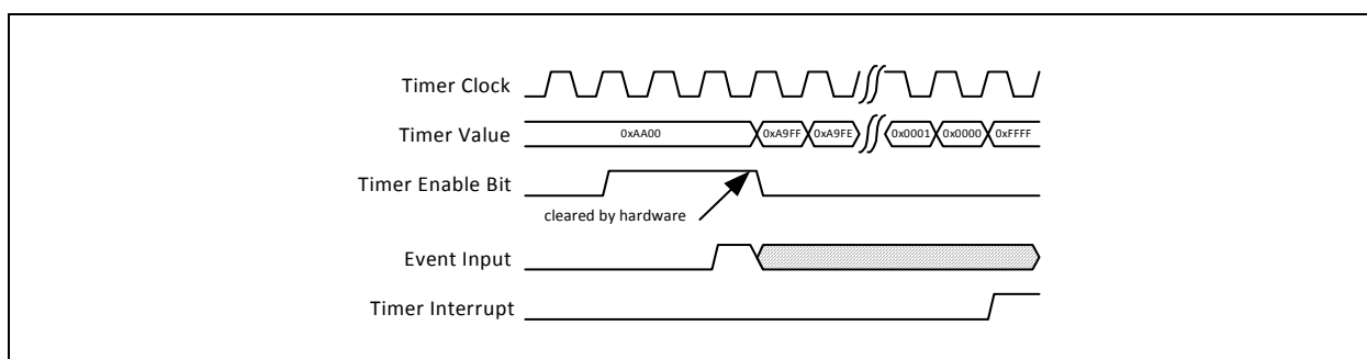
FIGURE 14-9: TIMER START BASED ON EXTERNAL EVENT
