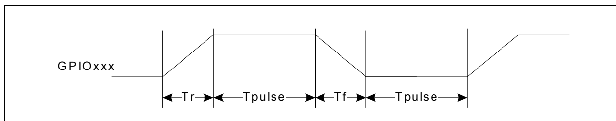
FIGURE 39-6: GPIO TIMING
