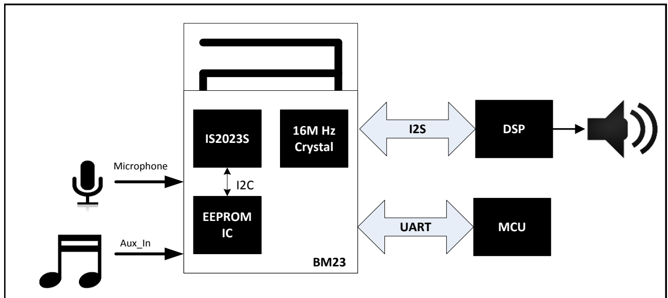
FIGURE 1-2: BM23 Typical Application
