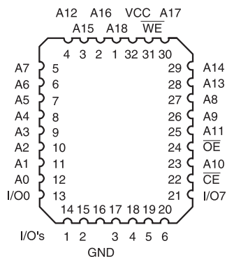
PLCC Top View
