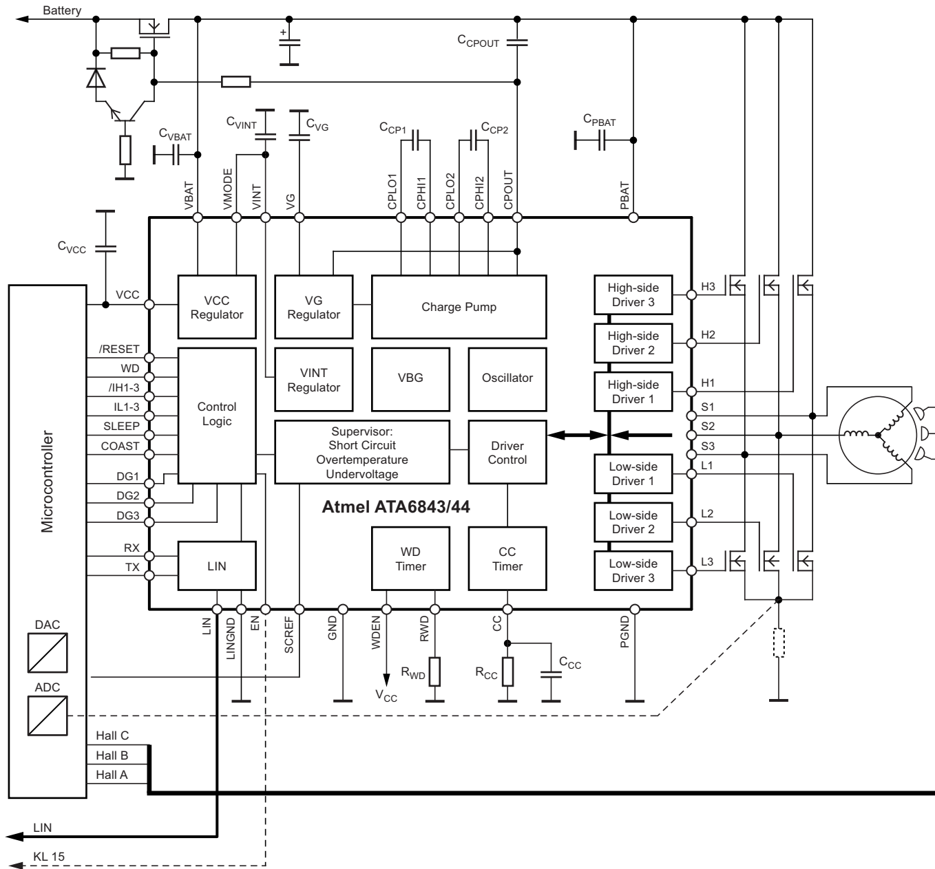
Figure 9-1. Typical Application
