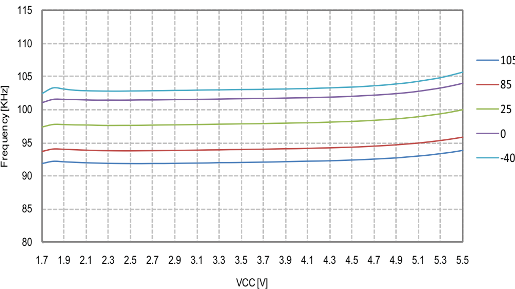
Figure 26-176. ULP 128kHz Oscillator, Frequency vs. Operating Voltage
