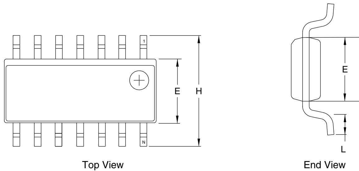
COMMON DIMENSIONS (Unit of Measure = mm/inches)
