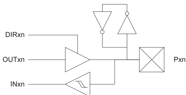
Figure 12-5. I/O Pin Configuration - Totem-pole with Bus-keeper
