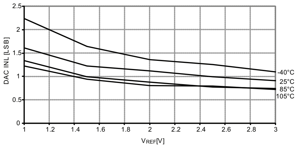
Figure 37-297. DAC INL error vs. V_{REF} .
