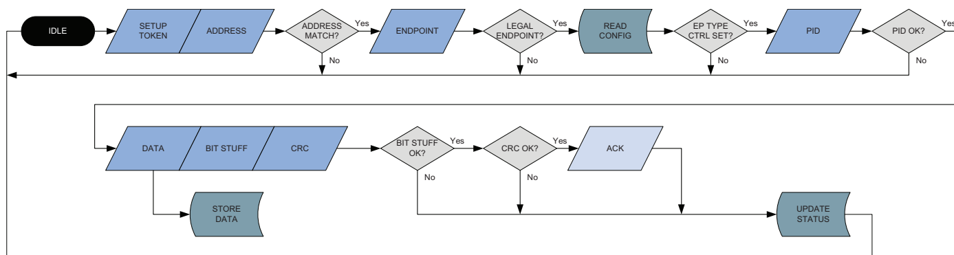
Figure 20-3. SETUP transaction.
