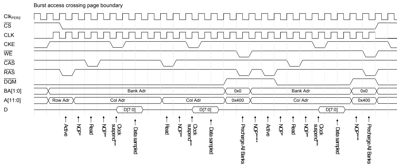
Figure 36-19. Burst access crossing page boundary
