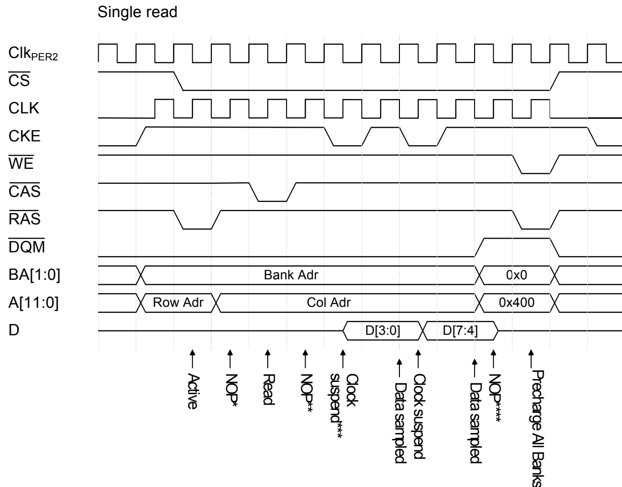
Figure 36-24. Single read
