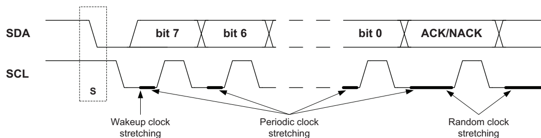
Figure 21-8. Clock stretching (1) .
