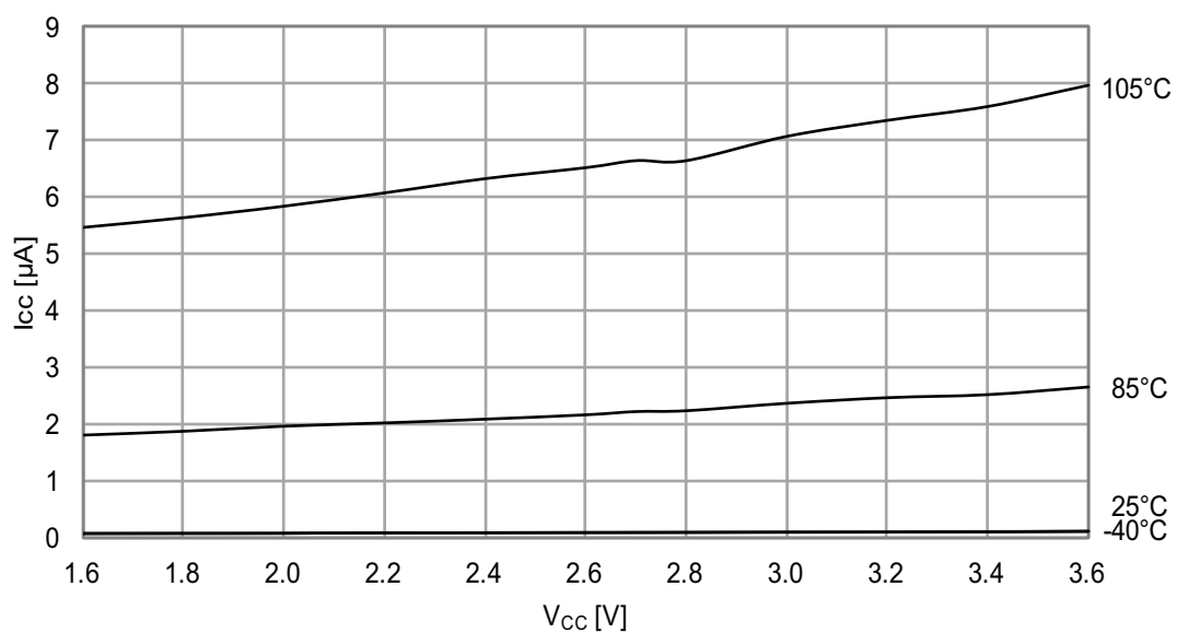
Figure 37-16. Power-down Mode Supply Current vs. V_{CC}
