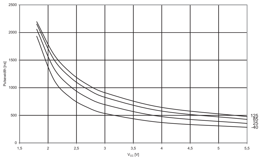
Figure 4-49. Minimum Reset Pulse Width vs. V_{CC}
