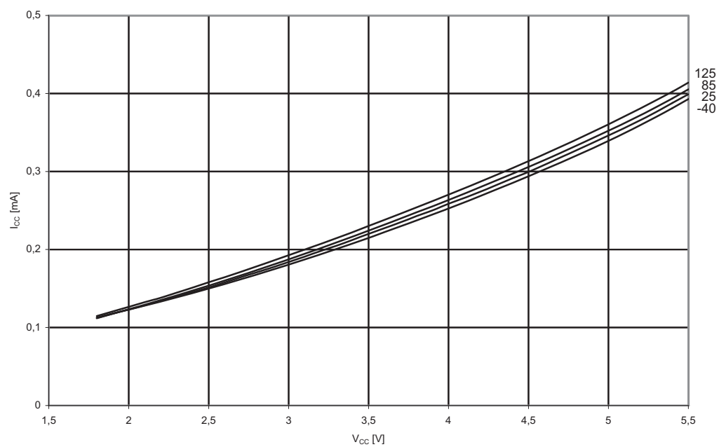
Figure 4-6. Idle Supply Current vs. V_{CC} (Internal Oscillator, 32kHz)
