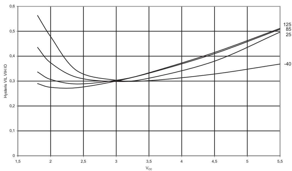
Figure 4-22. V_{IH}-V_{IL} : Input Hysteresis vs. V_{CC} (I/O Pin)
