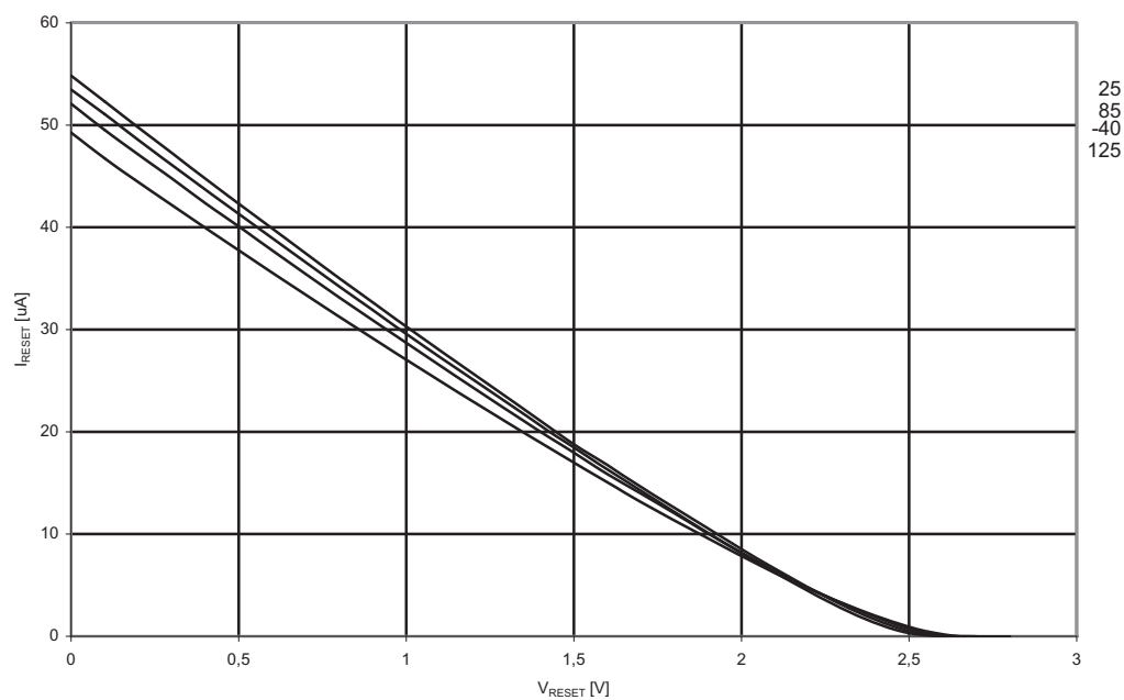
Figure 4-18. Reset Pull-up Resistor Current vs. Reset Pin Voltage ( V_{CC} = 2.7V )
