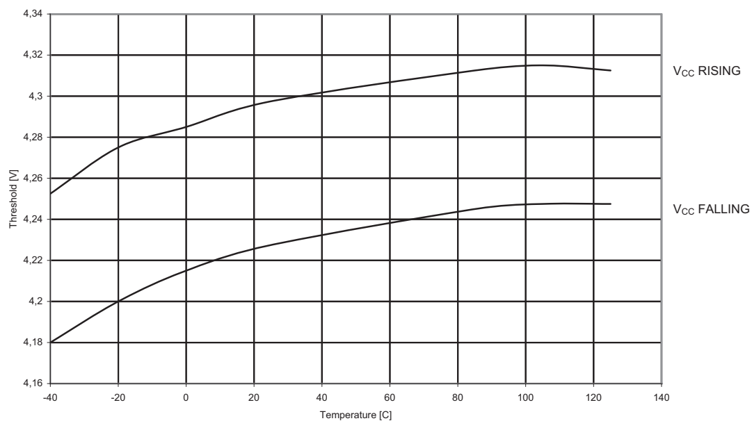
Figure 4-38. BOD Threshold vs Temperature (BODLEVEL = 4.3V)
