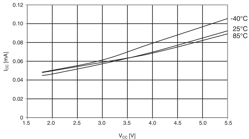
Figure 30-10. Atmel ATmega164A: Idle supply current vs. V_{CC} (internal RC oscillator, 128kHz).
