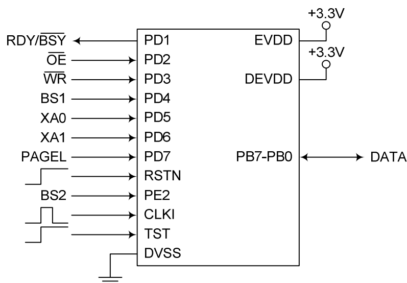
Figure 31-1. Parallel Programming (1)
