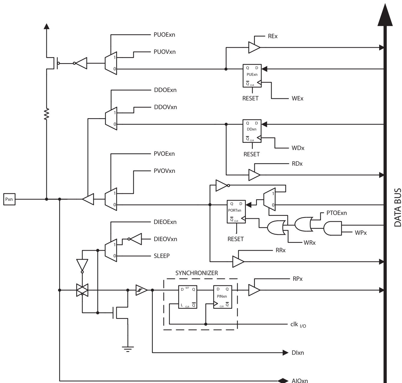
Figure 10-6. Alternate Port Functions (1)
