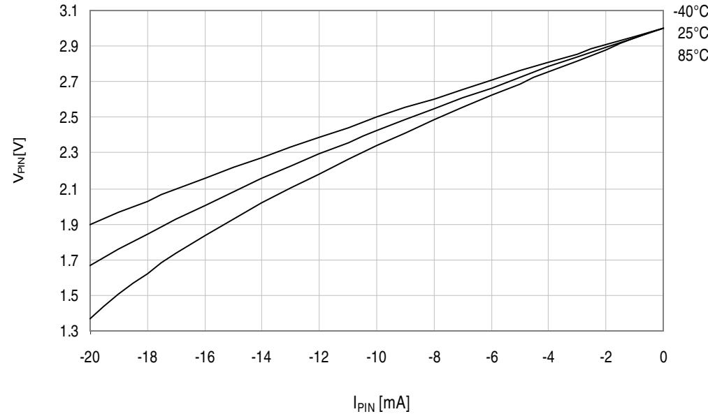
Figure 37-16.I/O pin output voltage vs. source current.
