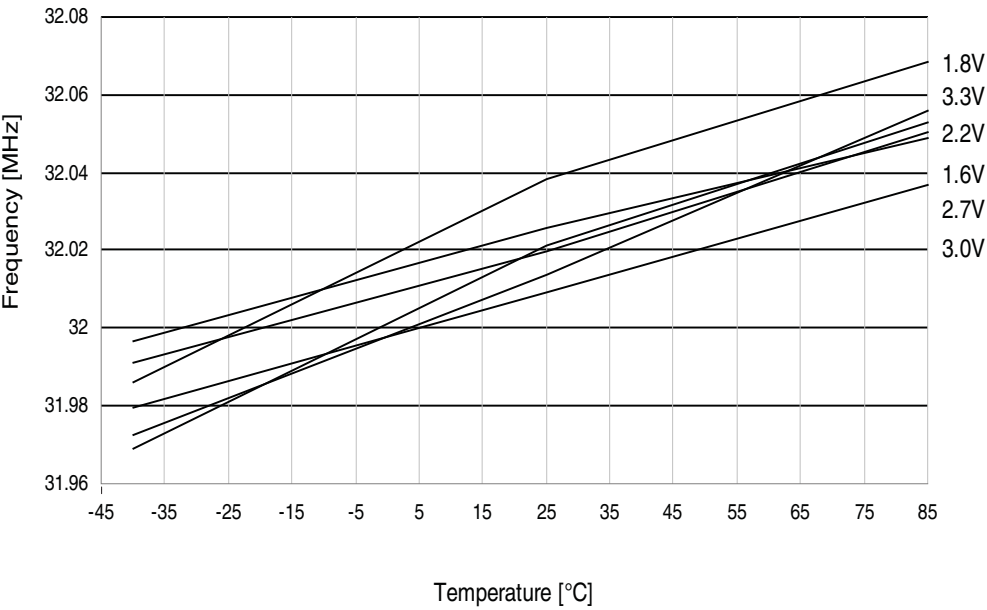
Figure 37-66. 32MHz internal oscillator frequency vs. temperature. DPLL enabled, from the 32.768kHz internal oscillator.
