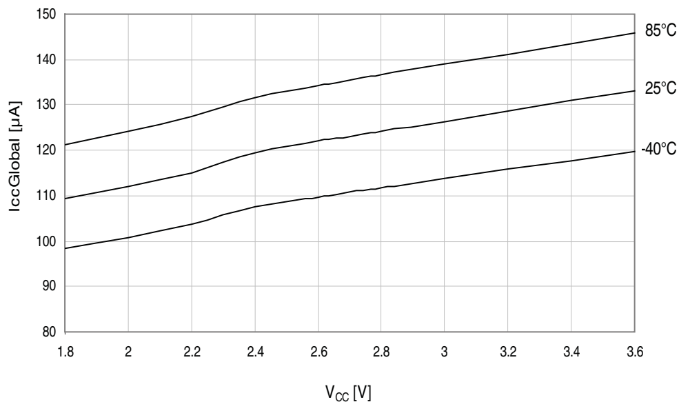
Figure 37-46.BOD current consumption vs. V_{CC} .
