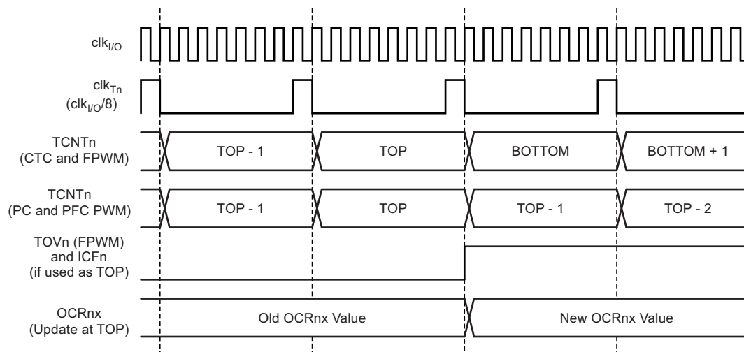
Figure 15-13. Timer/Counter Timing Diagram, with Prescaler ( f_{\text{clk\_I/O}}/8 )
