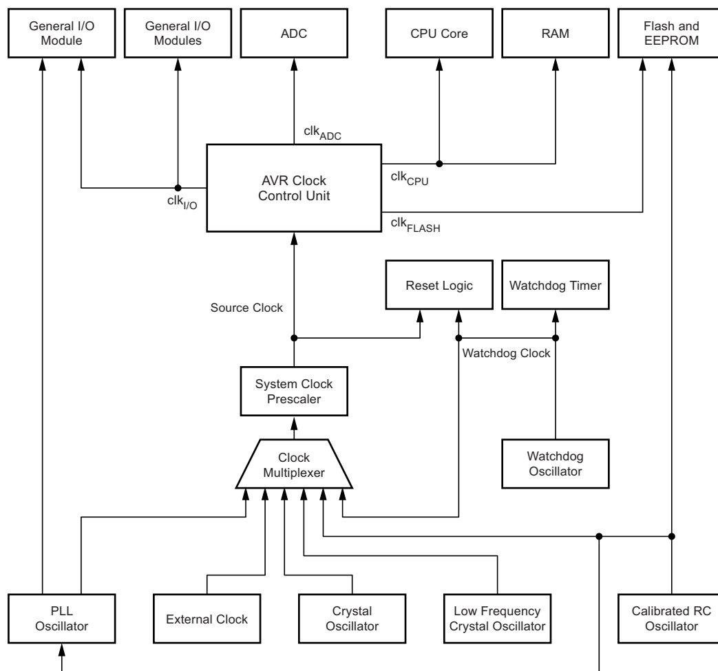
Figure 7-1. Clock Distribution
