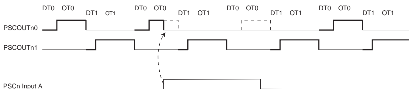
Figure 15-35. PSC behaviour versus PSCn Input A in Mode 14
