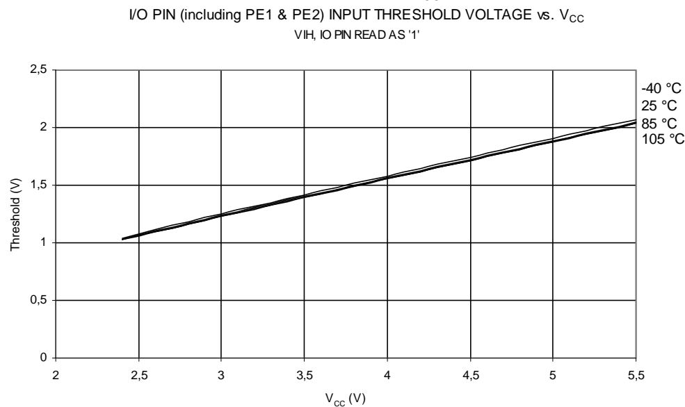
Figure 26-20. I/O Pin Input Threshold Voltage vs. V_{CC} ( V_{IH} , I/O Pin Read As '1')
