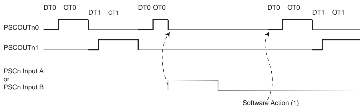
Figure 15-30. PSC behaviour versus PSCn Input A in Fault Mode 7
