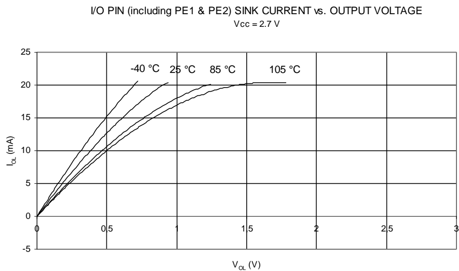
Figure 26-19. I/O Pin Sink Current vs. Output Voltage ( V_{CC} = 2.7V )
