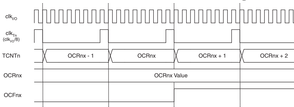
Figure 13-10. Timer/Counter Timing Diagram, Setting of \text{OCF0x} , with Prescaler ( f_{\text{clk}_{I/O}}/8 )
