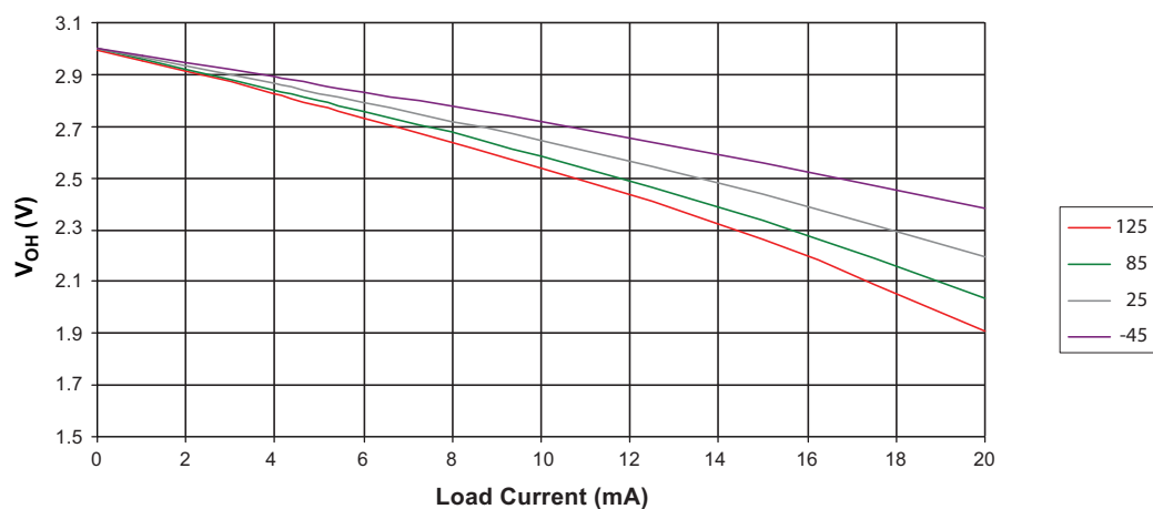
Figure 27-16. I/O Pin Output Voltage versus Source Current ( V_{CC} = 3.0V )
