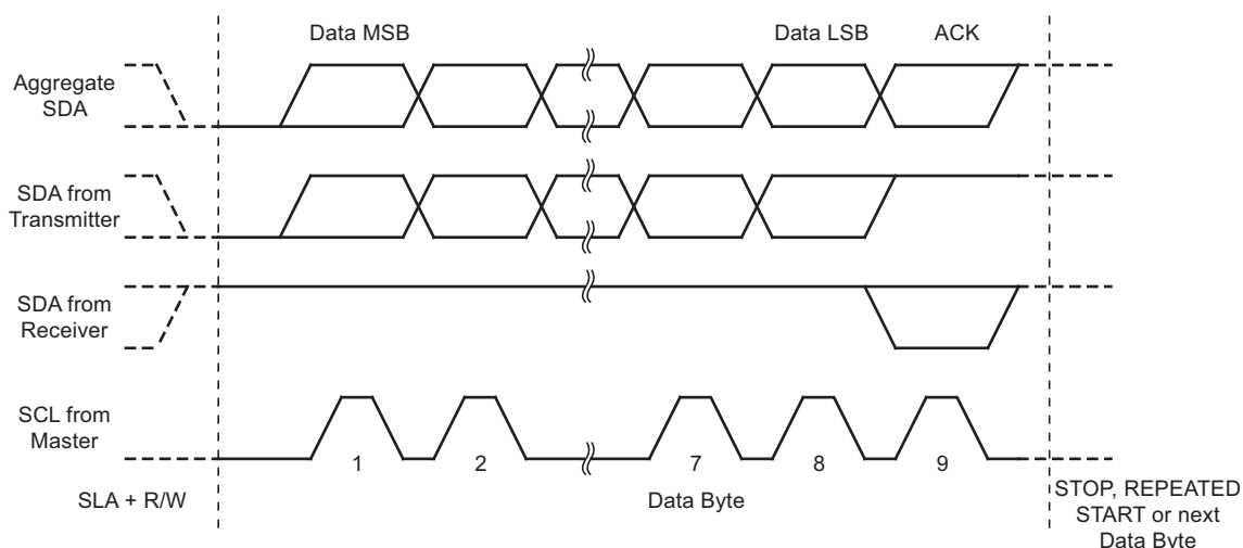
Figure 19-5. Data Packet Format
