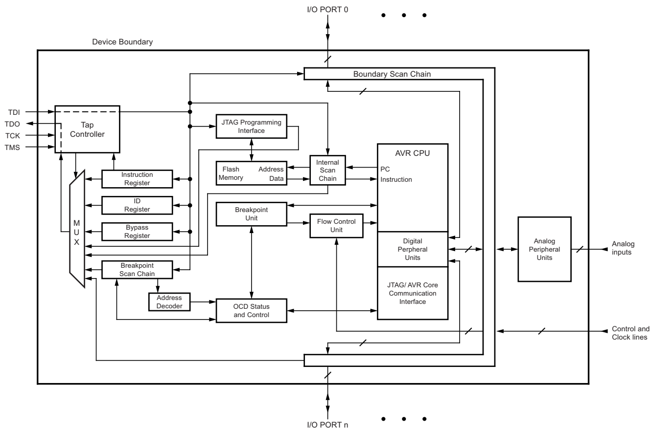
Figure 22-1. Block Diagram
