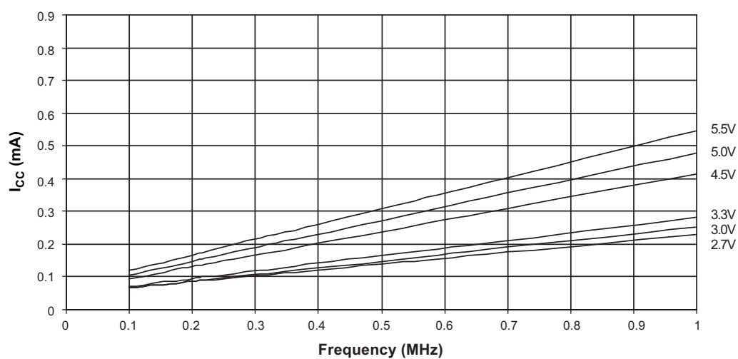
Figure 27-5. Idle Supply Current versus Frequency (0.1 - 1.0MHz) - Temperature = 25°C
