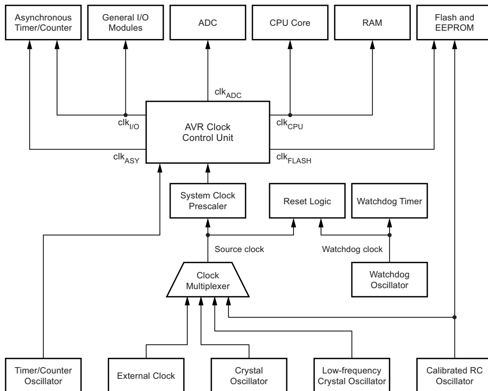
Figure 7-1. Clock Distribution
