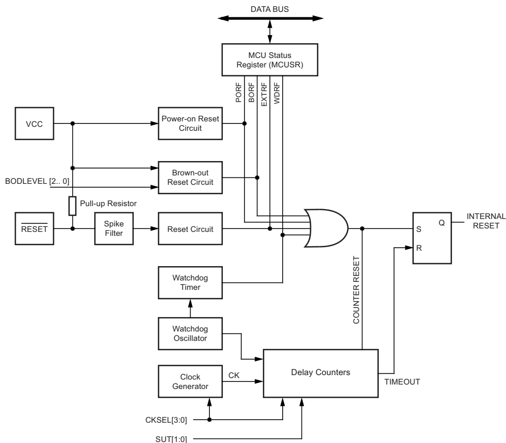
Figure 7-1. Reset Logic
