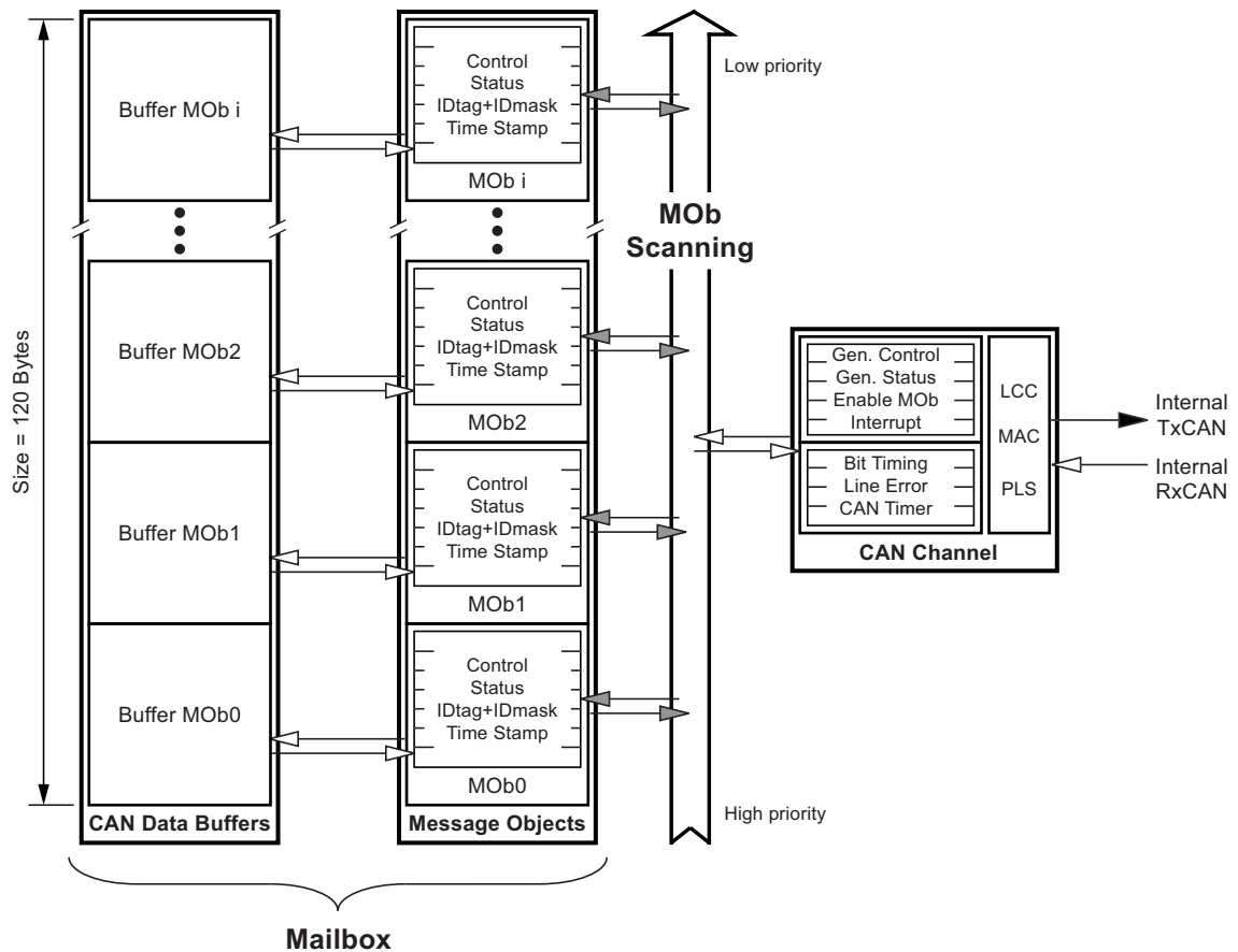
Figure 16-5. CAN Controller Structure
