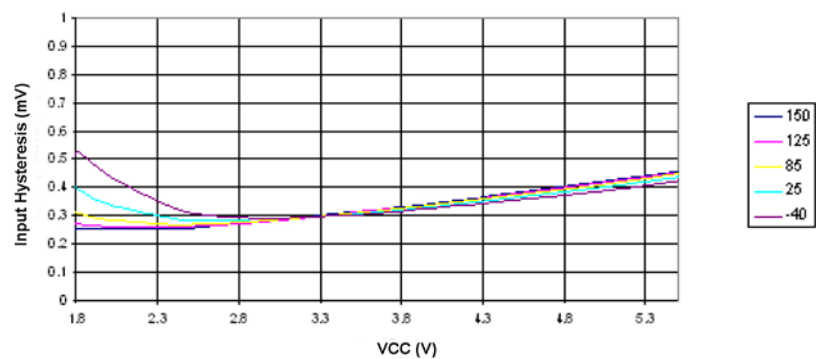
Figure 27-21. I/O Pin Input Hysteresis Voltage versus V_{CC}
