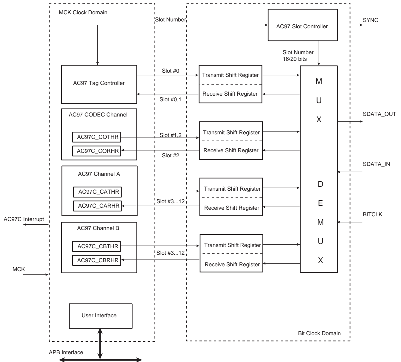
Figure 42-1. Functional Block Diagram
