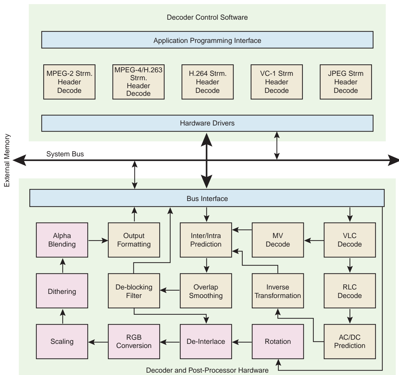
Figure 45-1. Block Diagram
