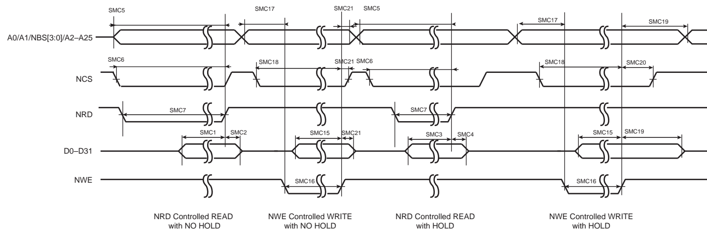
Figure 46-5. SMC Timings - NRD Controlled Read and NWE Controlled Write
