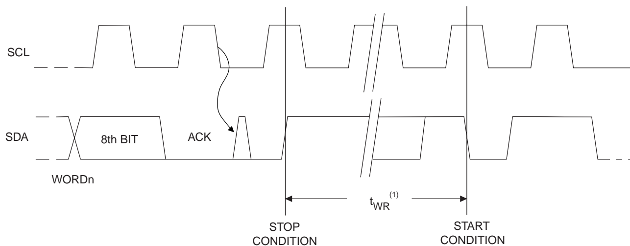
Figure 11-2. Write Cycle Timing
