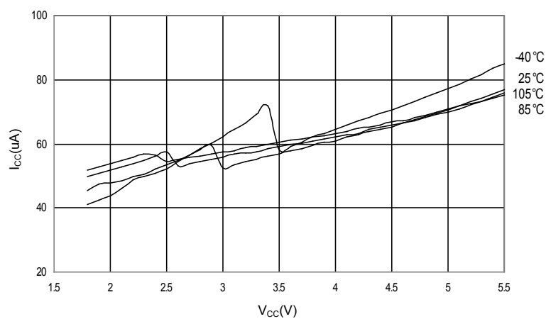
Figure 30-40. Analog Comparator Current vs. V_{CC}
