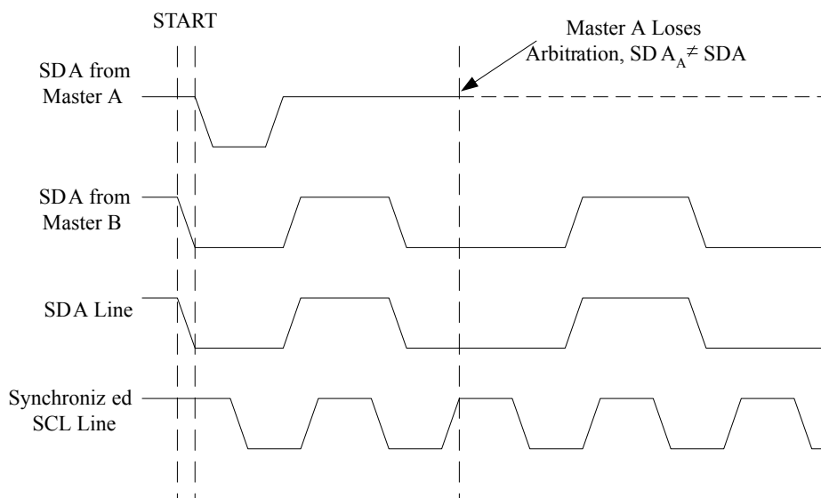
Figure 23-8. Arbitration Between Two Masters
