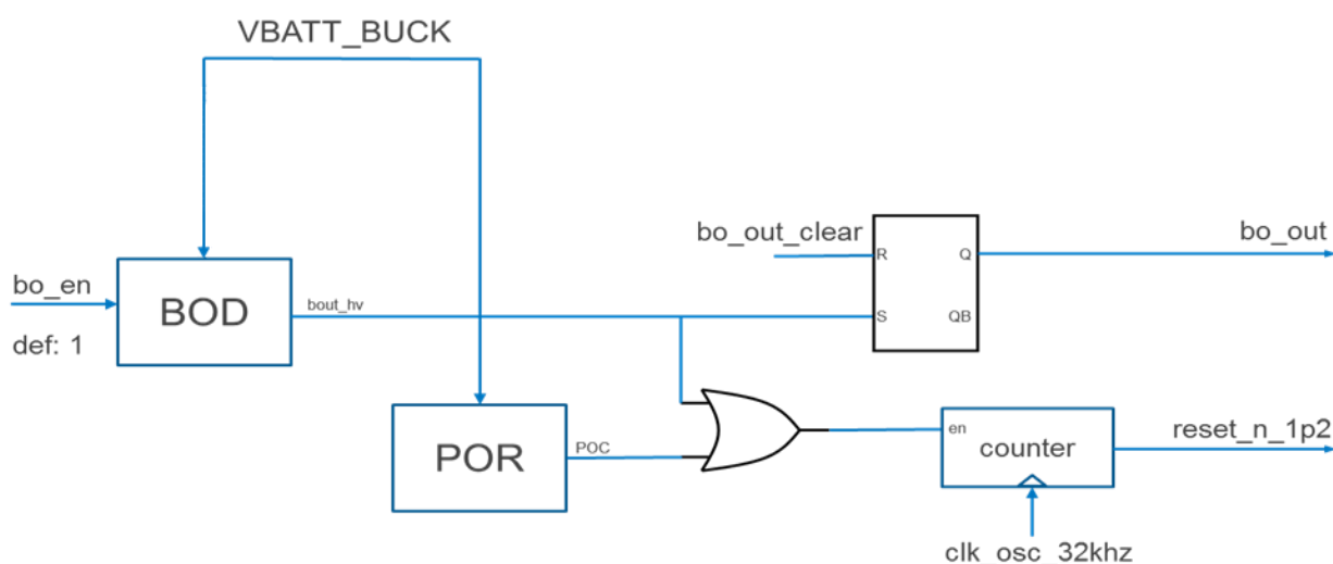
Figure 6-5. ATBTLC1000 POR and BOD Block Diagram
