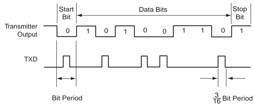
Figure 24-26. IrDA Modulation
