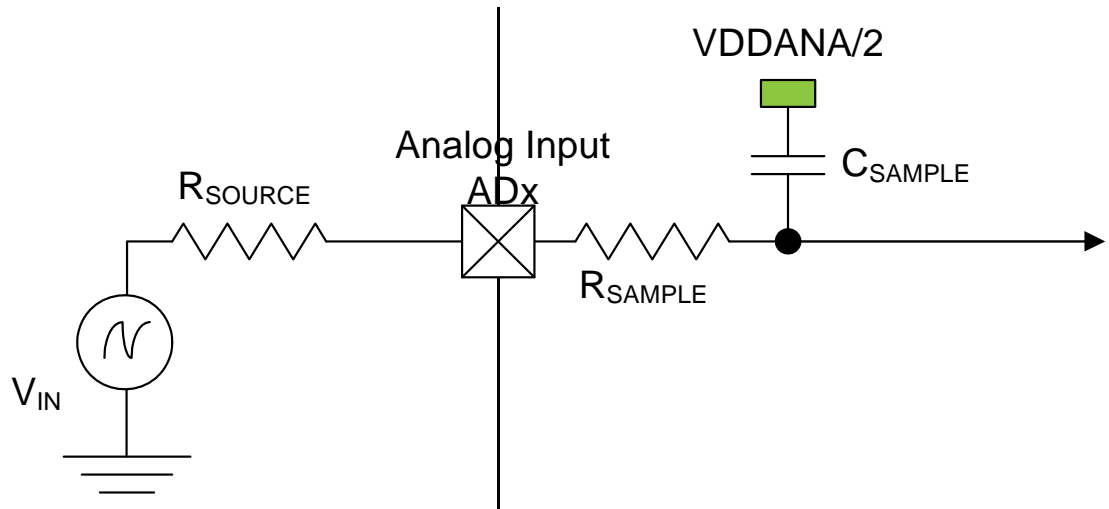
Figure 42-6. ADC Input
