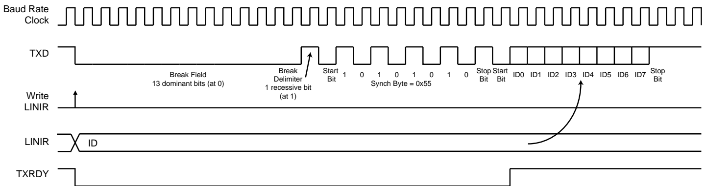
Figure 24-28. Header Transmission
