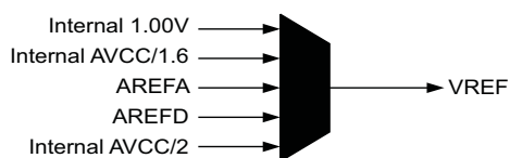
Figure 25-7. ADC Voltage Reference Selection
