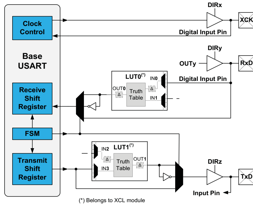
Figure 21-10.USART Encoding/Decoding Scheme
