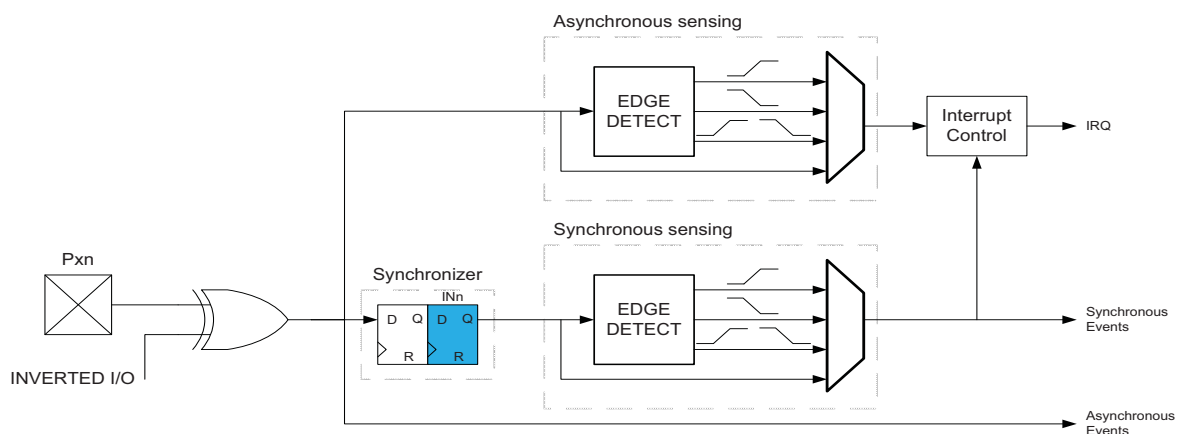
Figure 12-9. Input Sensing
