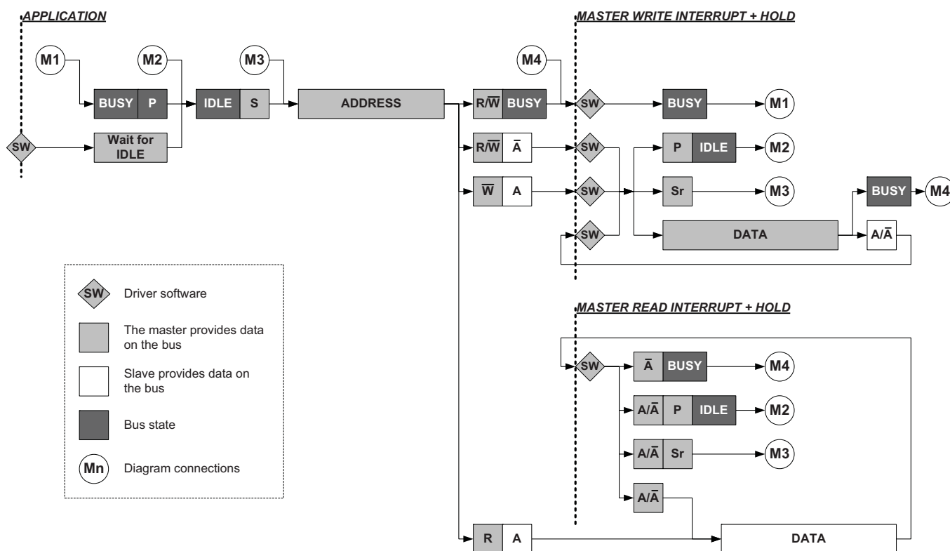
Figure 18-12.TWI Master Operation
