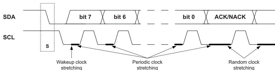
Figure 18-8. Clock Stretching (1)
