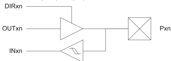
Figure 12-2. I/O Pin Configuration - Totem-pole (Push-pull)
