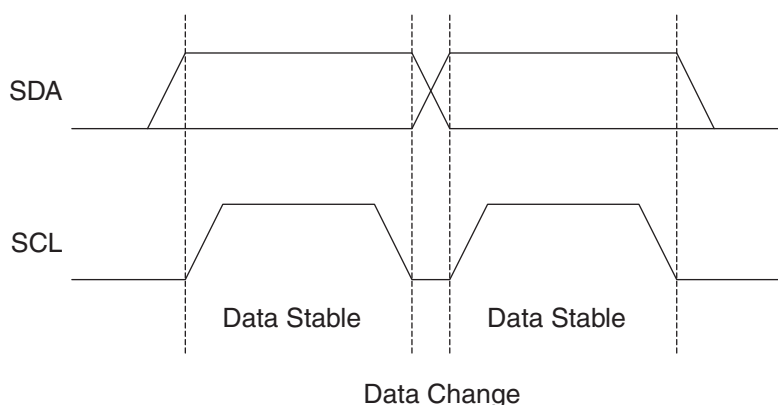
Figure 25-2. Data Validity
