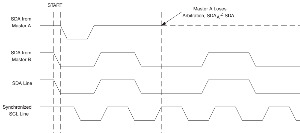
Figure 25-8. Arbitration between Two Masters
