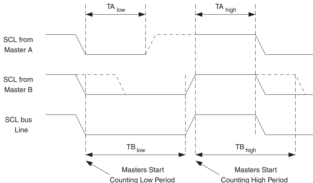
Figure 25-7. SCL Synchronization between Multiple Masters
