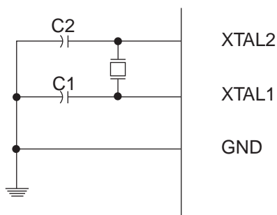
Figure 7-2. 32 kHz Crystal Oscillator Connections
