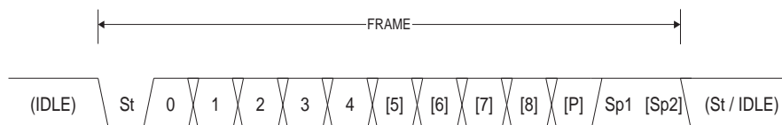
Figure 78. Frame Formats
