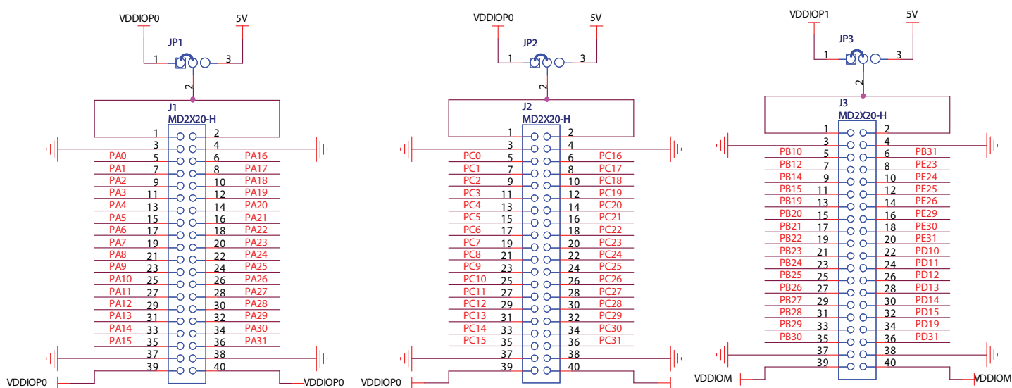
Figure 5-21. I/O Expansion
