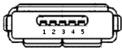
Figure 5-27. USB Host/Device MicroAB Connector J20
