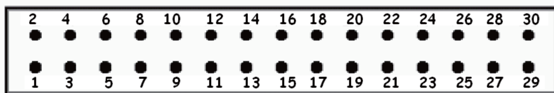
Figure 5-38. LCD Socket J21
