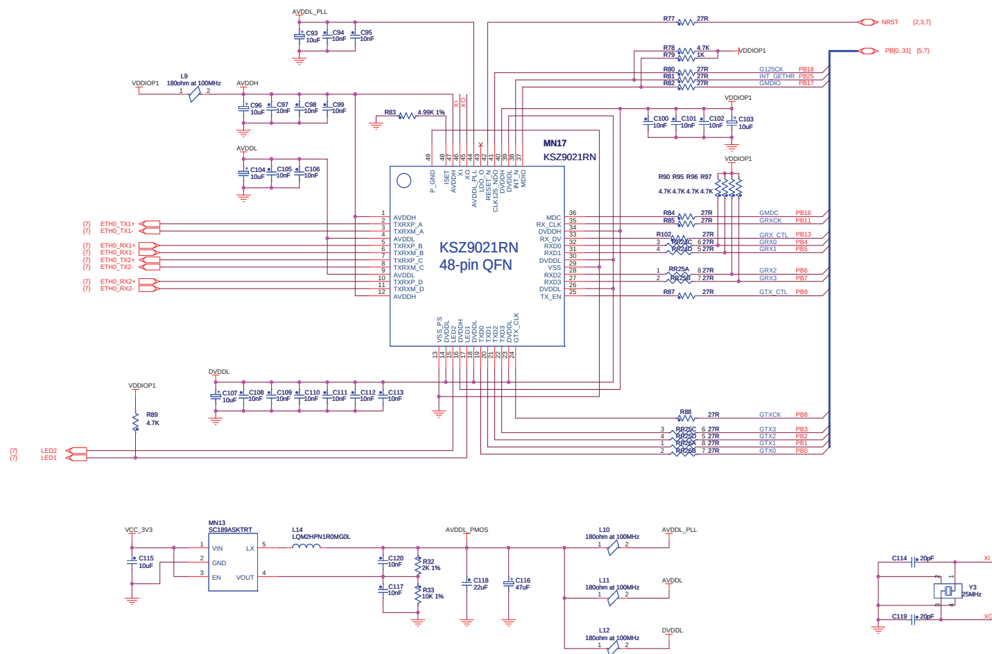
Figure 4-15. Embest/Flextronics GEthernet ETH0
