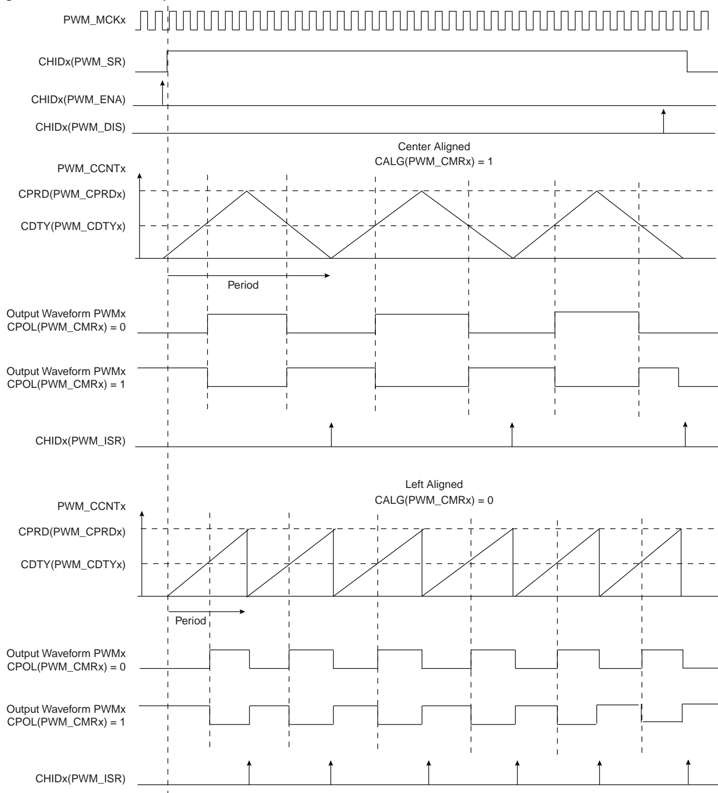
Figure 33-5. Waveform Properties
