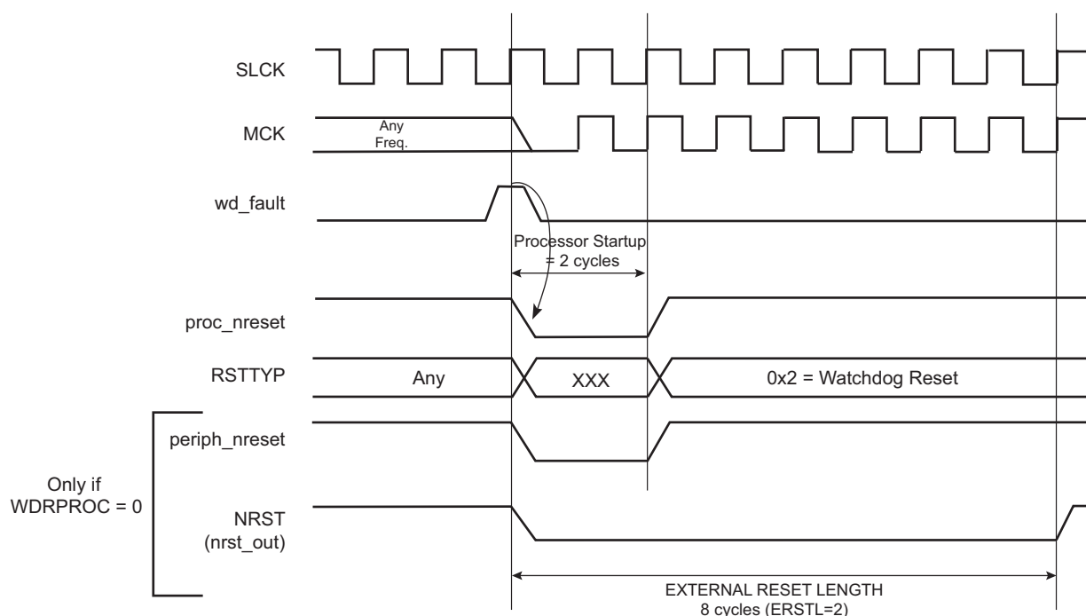
Figure 13-4. Watchdog Reset
