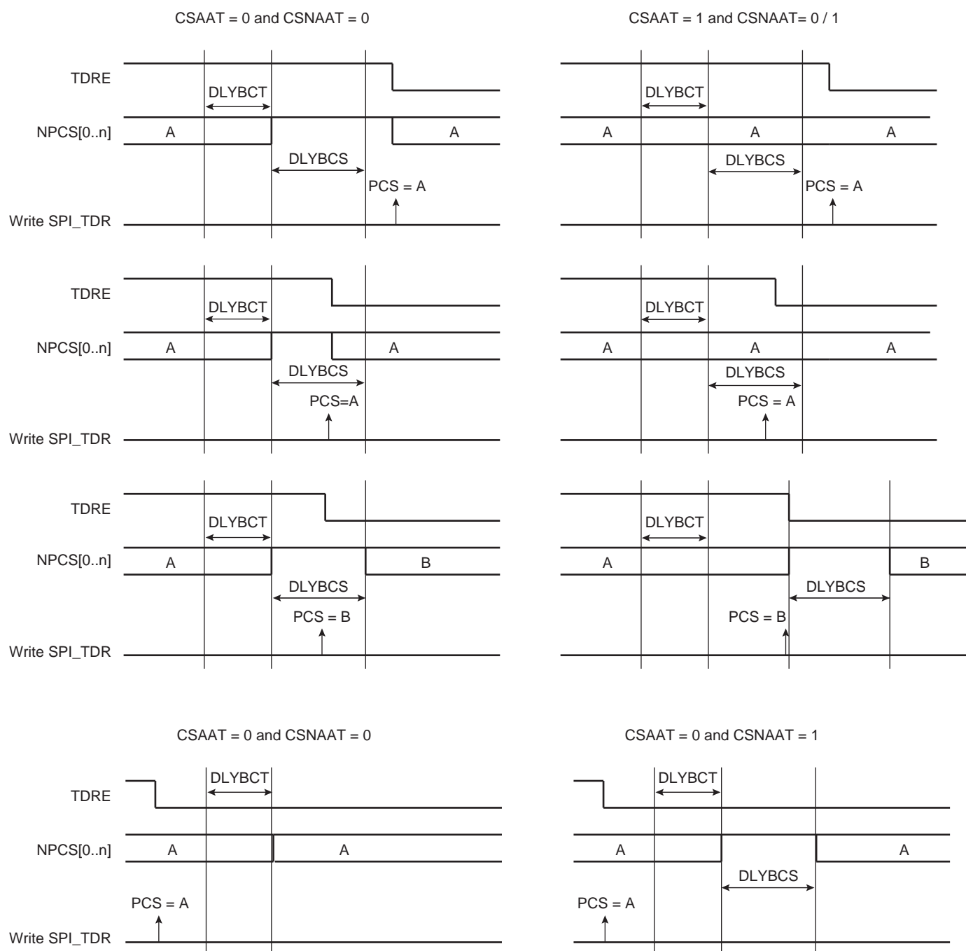
Figure 34-12. Peripheral Deselection
