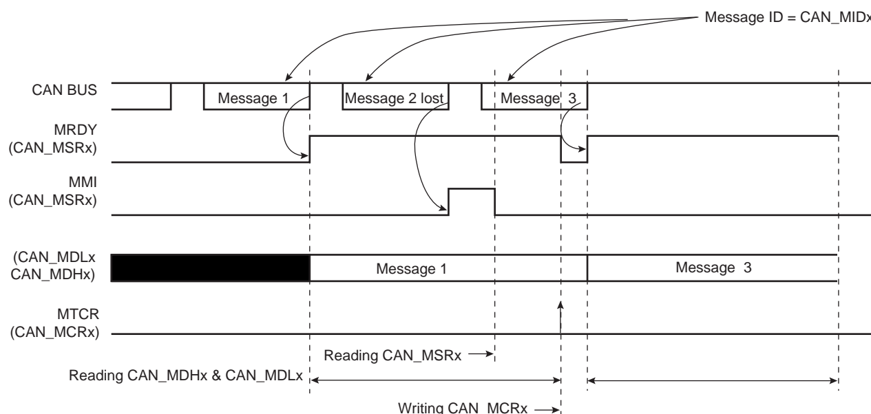
Figure 31-11. Receive Mailbox
