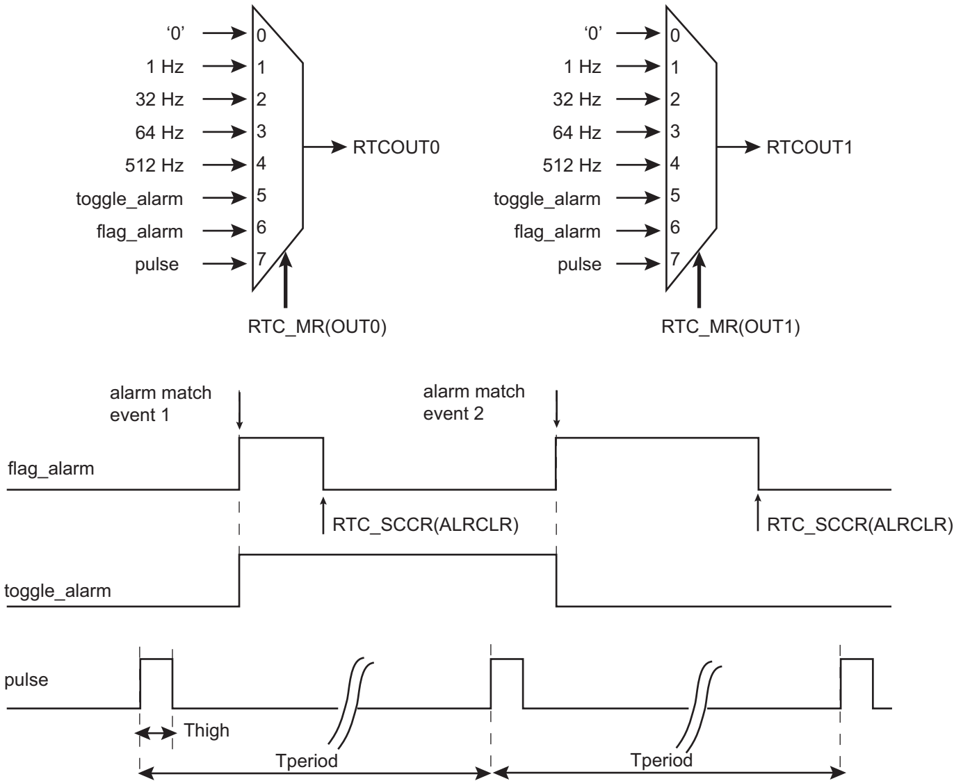
Figure 15-6. Waveform Generation
