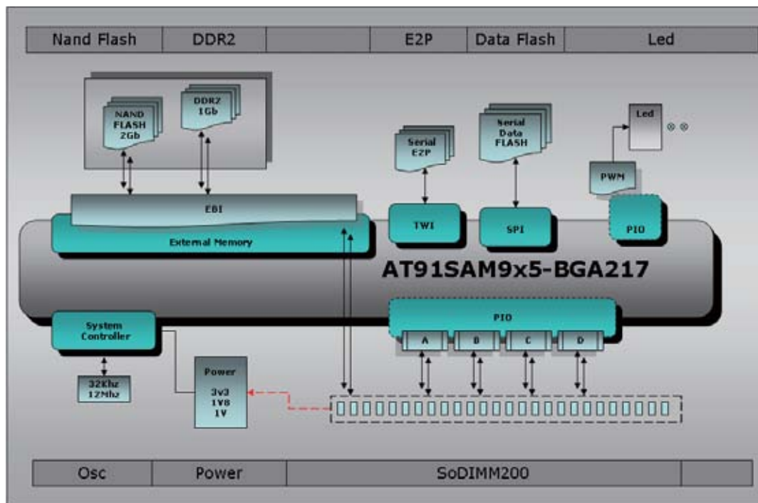
Figure 3-1. Board Architecture
