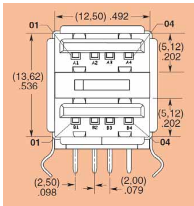
Figure 3-39. USB Type A Dual Port J19
